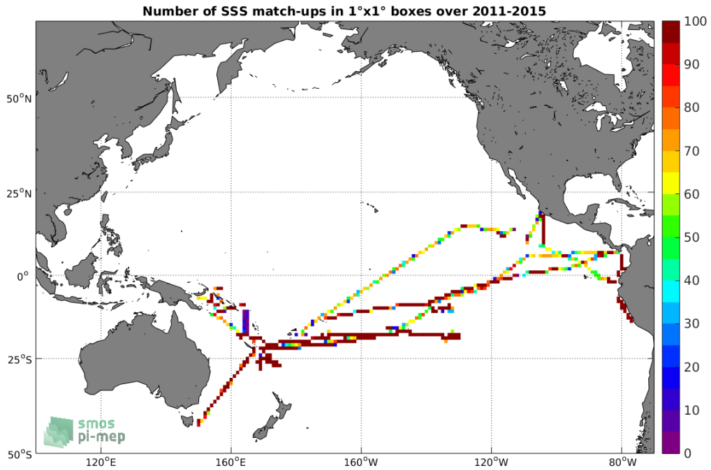
Figure 4: Number of SSS match-ups between TSG-GOSUD-Research-vessel SSS and the Aquarius-L3-OR-V5-7DAY-RUNNING-1DEG SSS product for the Pacific Ocean Pi-MEP region over 1°x1° boxes and for the full satellite product period.
