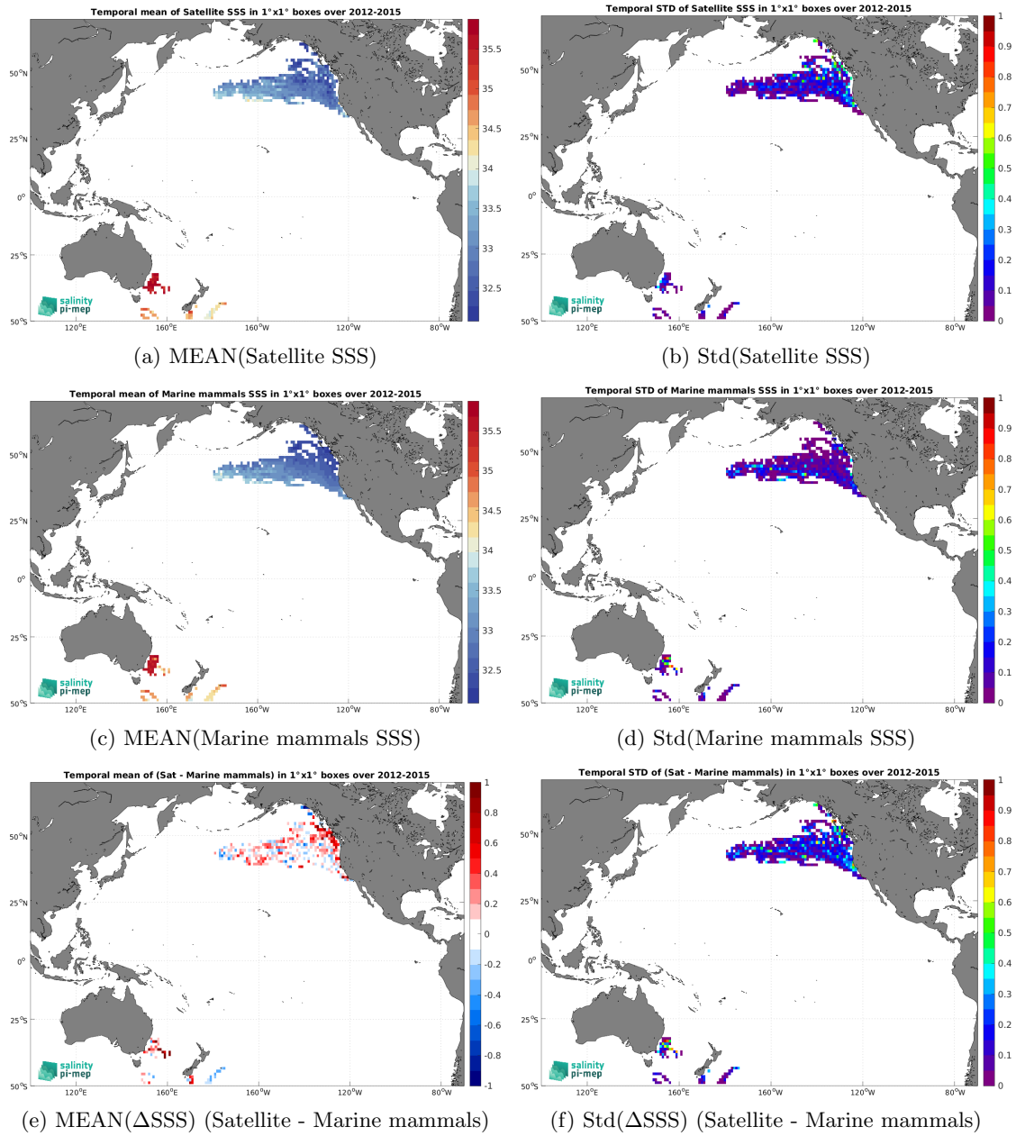
Figure 6: Temporal mean (left) and Std (right) of SSS from Aquarius SSS L3 OR v5 - 7-Day running (NASA-GSFC) (top), Marine mammals (middle), and of \Delta SSS (Satellite - Marine mammals). Only match-up pairs are used to generate these maps.
