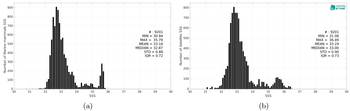
Figure 2: Histograms of SSS from Marine mammals (a) and Aquarius SSS L3 OR v5 - 7-Day running (NASA-GSFC) (b) considering all match-up pairs per bins of 0.1 over the Pacific Ocean Pi-MEP region and for the full satellite product period.
