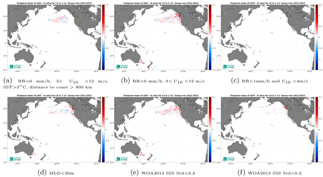
Figure 12: Temporal mean gridded over spatial boxes of size 1^\circ \times 1^\circ of \Delta SSS (Aquarius SSS L3 OR v5 - 7-Day running (NASA-GSFC) - Marine mammals) for 6 different subdatasets corresponding to:RR=0 mm/h, 3 < U_{10} < 12 m/s, SST > 5^\circ\text{C} , distance to coast > 800 km (a), RR=0 mm/h, 3 < U_{10} < 12 m/s (b), RR > 1 mm/h and U_{10} < 4 m/s (c),MLD < 20 m (d),WOA2013 SSS Std < 0.2 (e),WOA2013 SSS Std > 0.2 (f).
