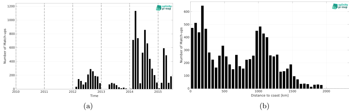
Figure 1: Number of match-ups between Marine mammals and Aquarius SSS L3 OR v5 - 7-Day running (NASA-GSFC) SSS as a function of time (a) and as function of the distance to coast (b) over the Pacific Ocean Pi-MEP region and for the full satellite product period.
