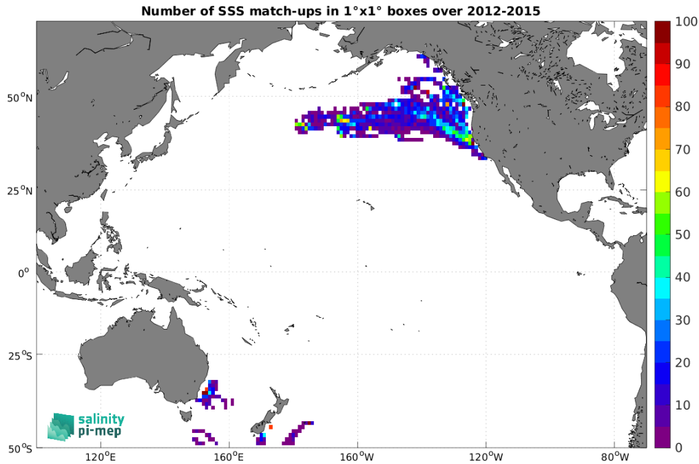
Figure 4: Number of SSS match-ups between Marine mammals SSS and the Aquarius SSS L3 OR v5 - 7-Day running (NASA-GSFC) SSS product for the Pacific Ocean Pi-MEP region over 1^\circ \times 1^\circ boxes and for the full satellite product period.
