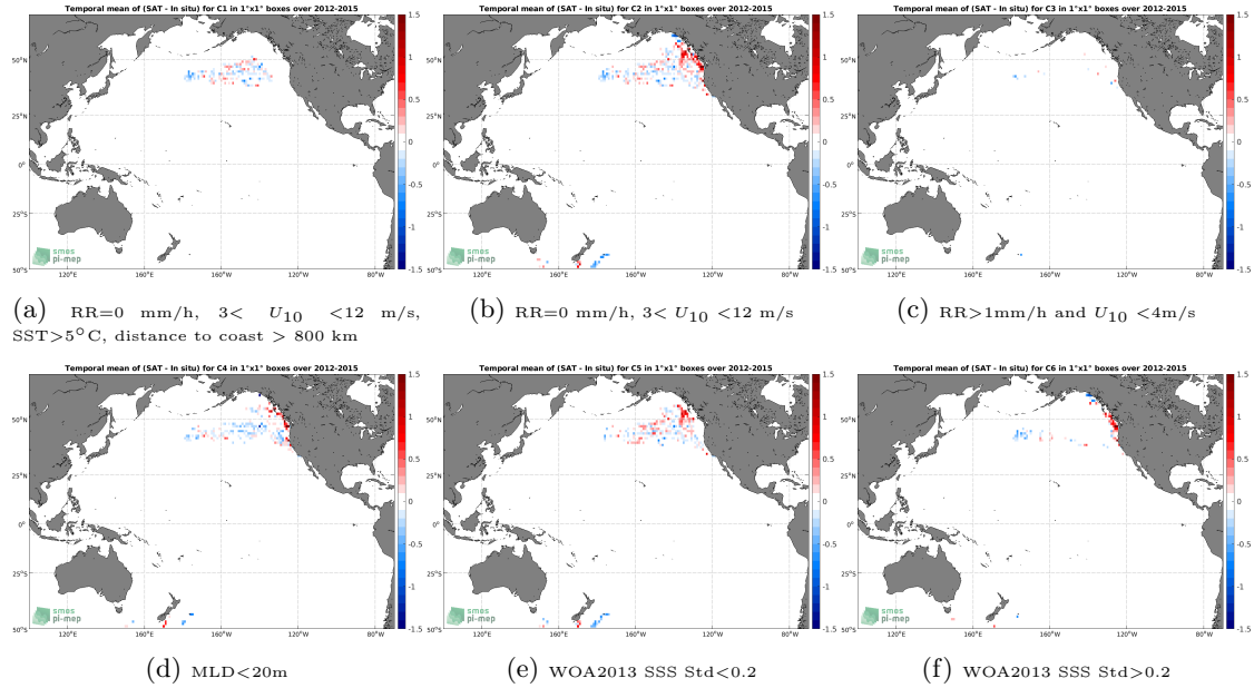
Figure 12: Temporal mean gridded over spatial boxes of size 1^\circ \times 1^\circ of \Delta SSS (Aquarius SSS L3 OR v5 - 7-Day running (NASA-GSFC) - Sea mammals) for 6 different subdatasets corresponding to:RR=0 mm/h, 3 < U_{10} < 12 m/s, SST >5^\circ\text{C} , distance to coast > 800 km (a), RR=0 mm/h, 3 < U_{10} < 12 m/s (b), RR >1 mm/h and U_{10} < 4 m/s (c),MLD <20 m (d),WOA2013 SSS Std <0.2 (e),WOA2013 SSS Std >0.2 (f).
