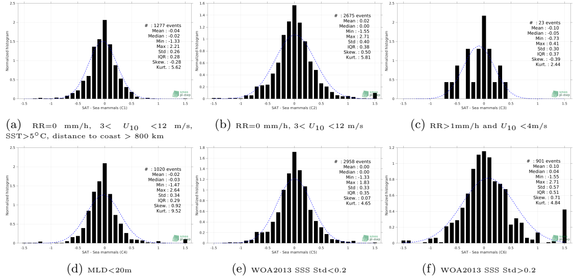
Figure 13: Normalized histogram of \Delta SSS (Aquarius SSS L3 OR v5 - 7-Day running (NASA-GSFC) - Sea mammals) for 6 different subdatasets corresponding to: RR=0 mm/h, 3 < U_{10} < 12 m/s, SST>5°C, distance to coast > 800 km (a), RR=0 mm/h, 3 < U_{10} < 12 m/s (b), RR>1mm/h and U_{10} < 4 m/s (c), MLD<20m (d), WOA2013 SSS Std<0.2 (e), WOA2013 SSS Std>0.2 (f).
