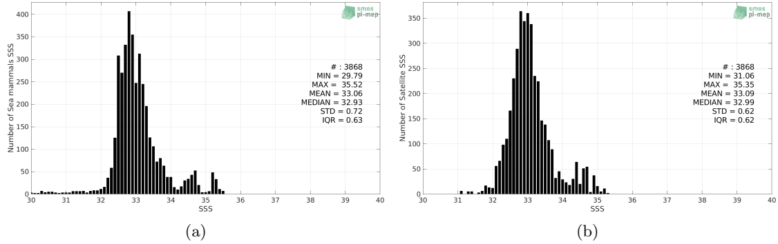
Figure 2: Histograms of SSS from Sea mammals (a) and Aquarius SSS L3 OR v5 - 7-Day running (NASA-GSFC) (b) considering all match-up pairs per bins of 0.1 over the Pacific Ocean Pi-MEP region and for the full satellite product period.
