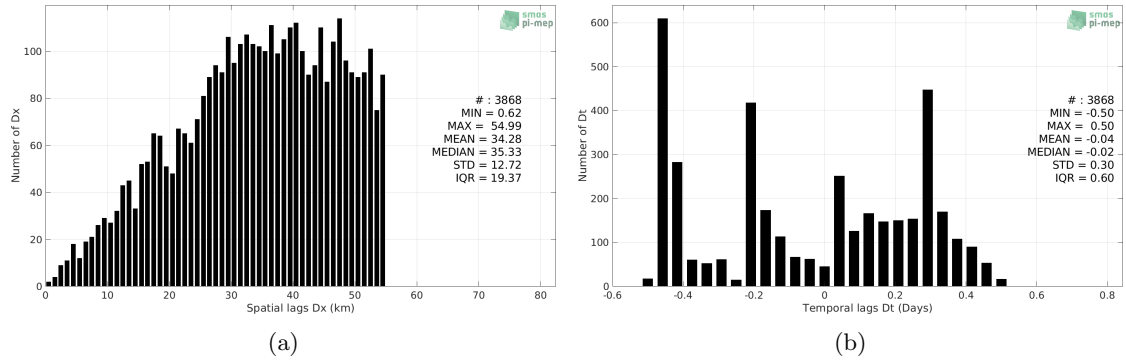
Figure 5: Histograms of the spatial (a) and temporal (b) lags between the location/time of the Sea mammals measurement and the date of the corresponding Aquarius SSS L3 OR v5 - 7-Day running (NASA-GSFC) SSS pixel.
