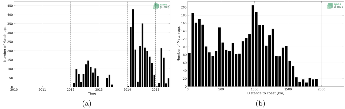
Figure 1: Number of match-ups between Sea mammals and Aquarius SSS L3 OR v5 - 7-Day running (NASA-GSFC) SSS as a function of time (a) and as function of the distance to coast (b) over the Pacific Ocean Pi-MEP region and for the full satellite product period.
