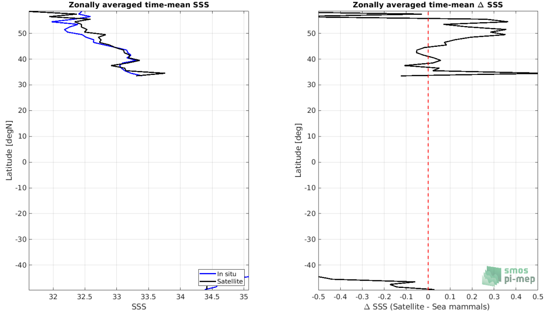
Figure 8: Left panel: Zonal mean SSS from Aquarius SSS L3 OR v5 - 7-Day running (NASA-GSFC) satellite product (black) and from Sea mammals (blue). Right panel: Zonal mean of \Delta SSS (Satellite - Sea mammals) for all the collected Pi-MEP match-up pairs estimated over the full satellite product period.
