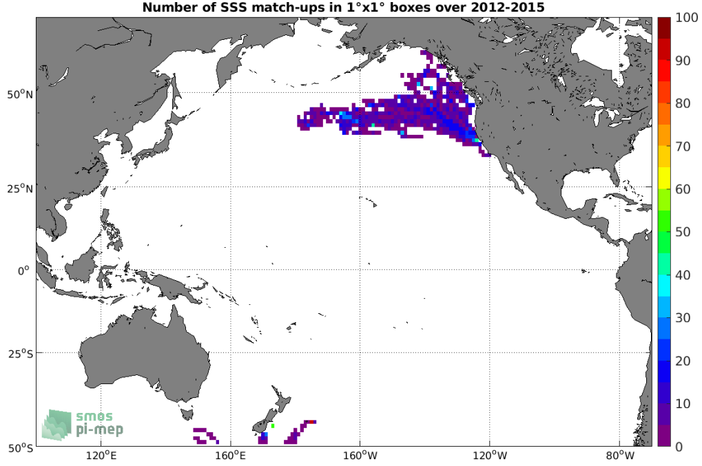
Figure 4: Number of SSS match-ups between Sea mammals SSS and the Aquarius SSS L3 OR v5 - 7-Day running (NASA-GSFC) SSS product for the Pacific Ocean Pi-MEP region over 1°x1° boxes and for the full satellite product period.
