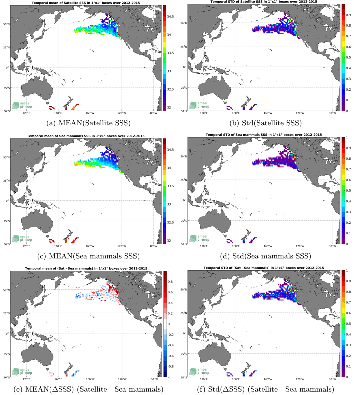
Figure 6: Temporal mean (left) and Std (right) of SSS from Aquarius SSS L3 OR v5 - 7-Day running (NASA-GSFC) (top), Sea mammals (middle), and of \Delta SSS (Satellite - Sea mammals). Only match-up pairs are used to generate these maps.
