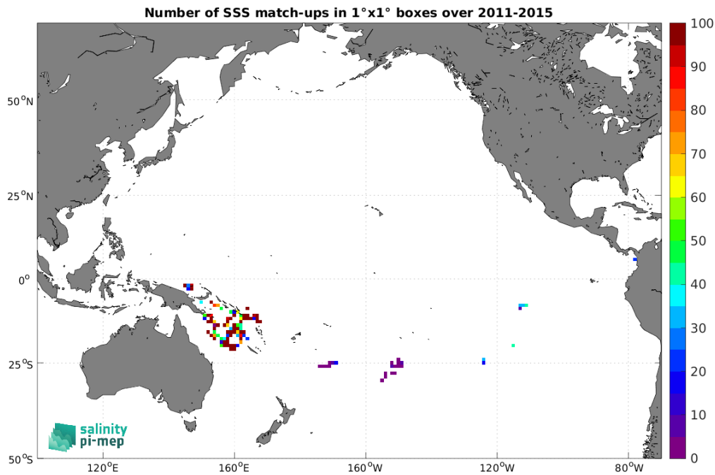
Figure 4: Number of SSS match-ups between Surface drifters SSS and the Aquarius SSS L3 OR v5 - 7-Day running (NASA-GSFC) SSS product for the Pacific Ocean Pi-MEP region over 1^\circ \times 1^\circ boxes and for the full satellite product period.
