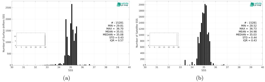
Figure 3: Histograms of SSS from Surface drifters (a) and Aquarius SSS L3 OR v5 - 7-Day running (NASA-GSFC) (b) considering all match-up pairs per bins of 0.1 over the Pacific Ocean Pi-MEP region and for the full satellite product period.
