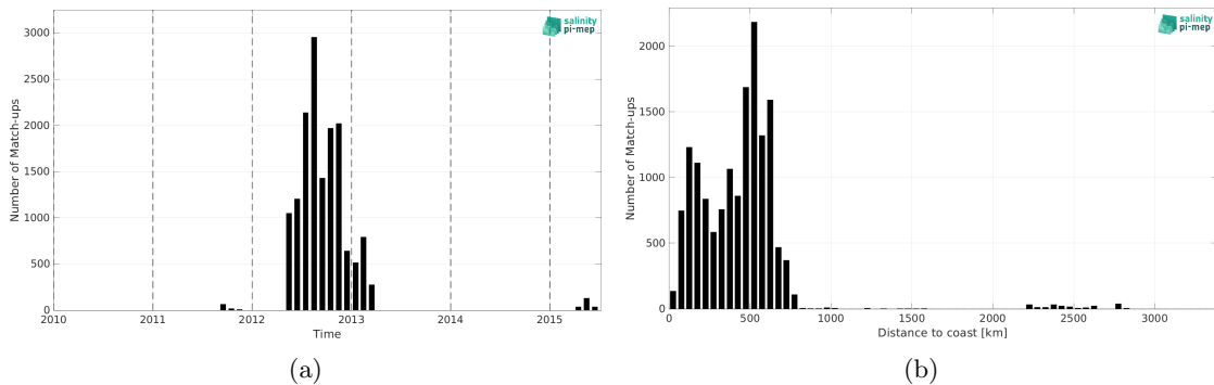
Figure 2: Number of match-ups between Surface drifters and Aquarius SSS L3 OR v5 - 7-Day running (NASA-GSFC) SSS as a function of time (a) and as function of the distance to coast (b) over the Pacific Ocean Pi-MEP region and for the full satellite product period.
