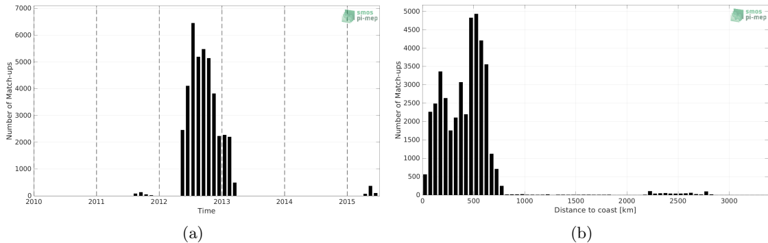
Figure 1: Number of match-ups between Surface drifters and Aquarius SSS L3 OR v5 - 7-Day running (NASA-GSFC) SSS as a function of time (a) and as function of the distance to coast (b) over the Pacific Ocean Pi-MEP region and for the full satellite product period.
