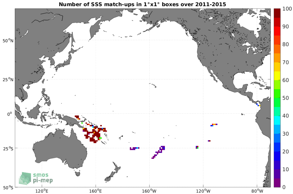
Figure 3: Number of SSS match-ups between Surface drifters SSS and the Aquarius SSS L3 OR v5 - 7-Day running (NASA-GSFC) SSS product for the Pacific Ocean Pi-MEP region over 1^\circ \times 1^\circ boxes and for the full satellite product period.
