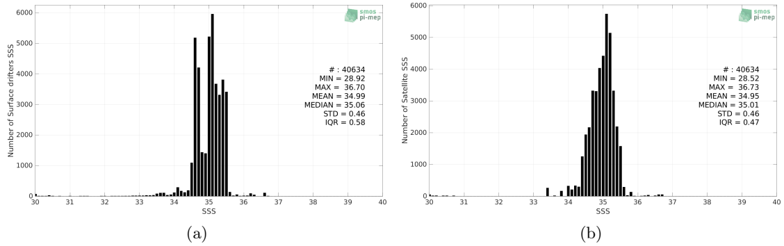
Figure 2: Histograms of SSS from Surface drifters (a) and Aquarius SSS L3 OR v5 - 7-Day running (NASA-GSFC) (b) considering all match-up pairs per bins of 0.1 over the Pacific Ocean Pi-MEP region and for the full satellite product period.
