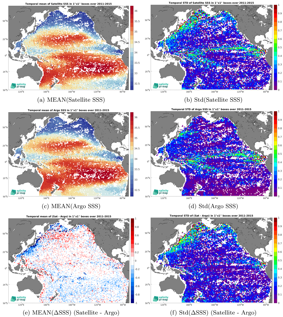
Figure 7: Temporal mean (left) and Std (right) of SSS from Aquarius SSS L3 OR v5 - 7-Day running (NASA-GSFC) (top), Argo (middle), and of \Delta SSS (Satellite - Argo). Only match-up pairs are used to generate these maps.
