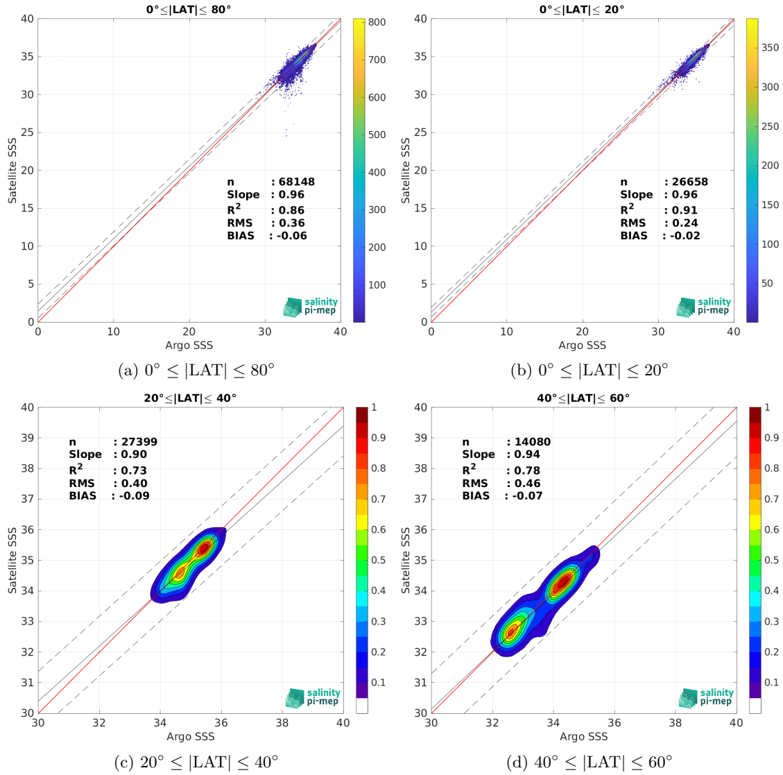
Figure 10: Contour maps of the concentration of Aquarius SSS L3 OR v5 - 7-Day running (NASA-GSFC) SSS ( y -axis) versus Argo SSS ( x -axis) at match-up pairs for different latitude bands. For each plot, the red line shows x=y . The black thin and dashed lines indicate a linear fit through the data cloud and the \pm 95\% confidence levels, respectively. The number match-up pairs n , the slope and R^2 coefficient of the linear fit, the root mean square (RMS) and the mean bias between satellite and in situ data are indicated for each latitude band in each plots.
