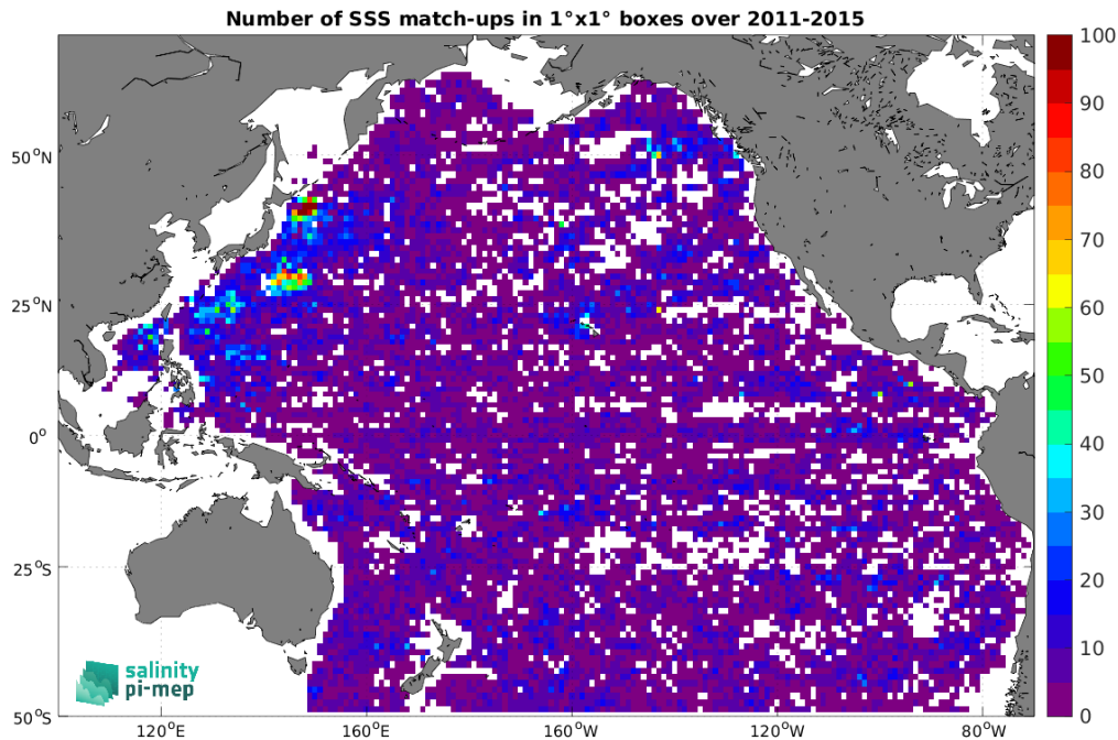
Figure 5: Number of SSS match-ups between Argo SSS and the Aquarius SSS L3 OR v5 - 7-Day running (NASA-GSFC) SSS product for the Pacific Ocean Pi-MEP region over 1^\circ \times 1^\circ boxes and for the full satellite product period.
