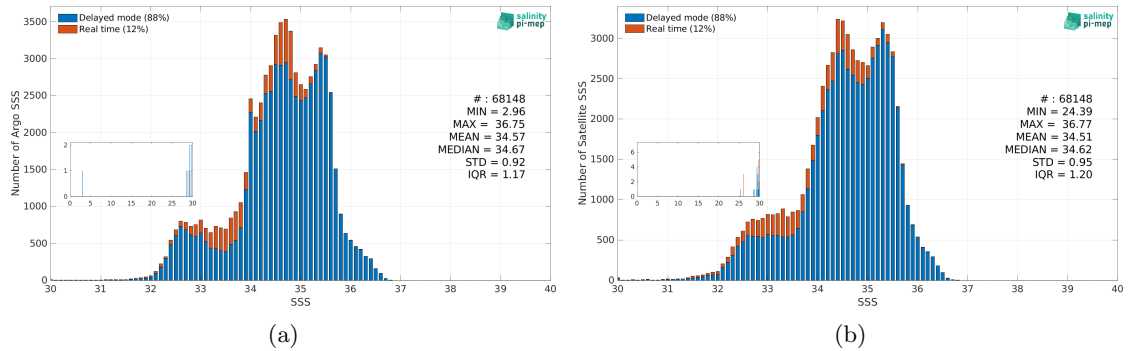
Figure 3: Histograms of SSS from Argo (a) and Aquarius SSS L3 OR v5 - 7-Day running (NASA-GSFC) (b) considering all match-up pairs per bins of 0.1 over the Pacific Ocean Pi-MEP region and for the full satellite product period.
