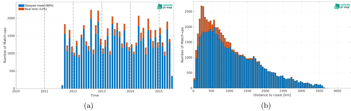
Figure 2: Number of match-ups between Argo and Aquarius SSS L3 OR v5 - 7-Day running (NASA-GSFC) SSS as a function of time (a) and as function of the distance to coast (b) over the Pacific Ocean Pi-MEP region and for the full satellite product period.
