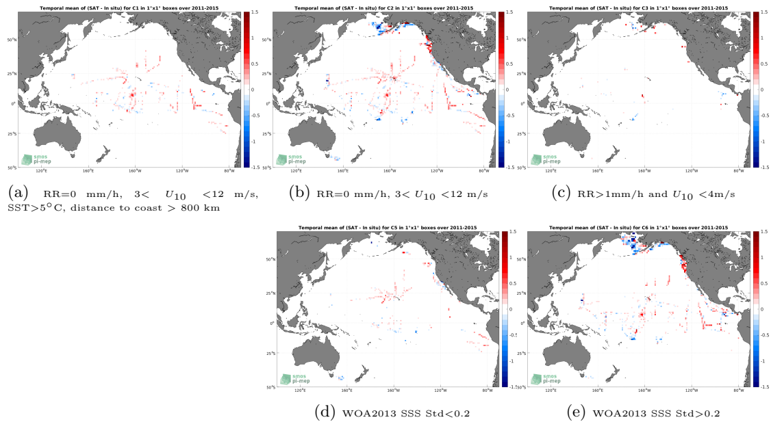
Figure 12: Temporal mean gridded over spatial boxes of size 1^\circ \times 1^\circ of \Delta SSS (Aquarius SSS L3 OR v5 - 7-Day running - Rain mask (NASA-GSFC) - TSG (SAMOS)) for 5 different subdatasets corresponding to:RR=0 mm/h, 3 < U_{10} < 12 m/s, SST >5^\circ\text{C} , distance to coast > 800 km (a), RR=0 mm/h, 3 < U_{10} < 12 m/s (b), RR >1 mm/h and U_{10} < 4 m/s (c), WOA2013 SSS Std <0.2 (d), WOA2013 SSS Std >0.2 (e).
