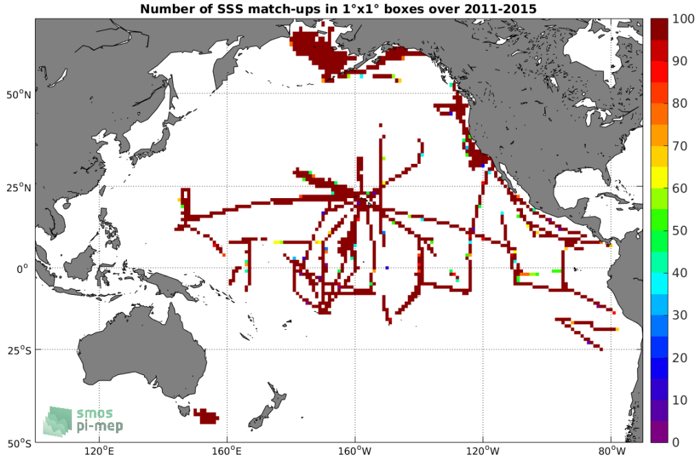
Figure 4: Number of SSS match-ups between TSG-SAMOS SSS and the Aquarius-L3-OR-V5-7DAY-RUNNING-RAIN-MASK-1DEG SSS product for the Pacific Ocean Pi-MEP region over 1°x1° boxes and for the full satellite product period.
