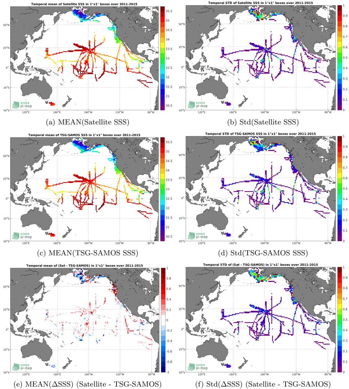
Figure 6: Temporal mean (left) and Std (right) of SSS from Aquarius-L3-OR-V5-7DAY-RUNNING-RAIN-MASK-1DEG (top), TSG-SAMOS (middle), and of \Delta SSS (Satellite - TSG-SAMOS). Only match-up pairs are used to generate these maps.
