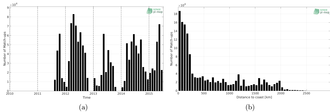
Figure 1: Number of match-ups between TSG-SAMOS and Aquarius-L3-OR-V5-7DAY-RUNNING-RAIN-MASK-1DEG SSS as a function of time (a) and as function of the distance to coast (b) over the Pacific Ocean Pi-MEP region and for the full satellite product period.
