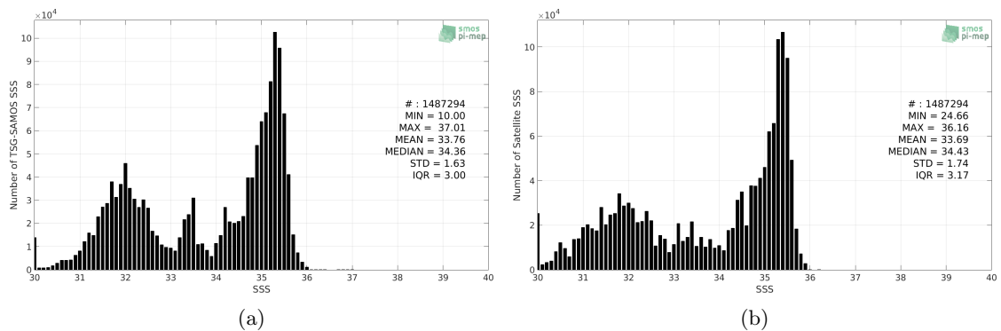
Figure 2: Histograms of SSS from TSG-SAMOS (a) and Aquarius-L3-OR-V5-7DAY-RUNNING-RAIN-MASK-1DEG (b) considering all match-up pairs per bins of 0.1 over the Pacific Ocean Pi-MEP region and for the full satellite product period.
