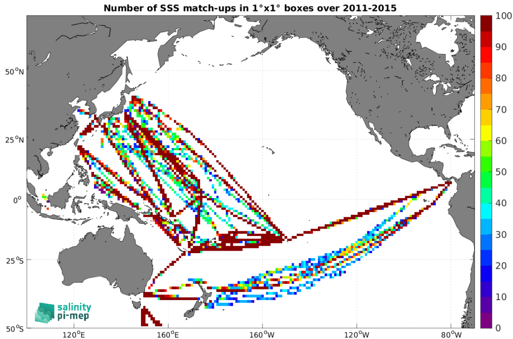
Figure 5: Number of SSS match-ups between TSG (LEGOS-DM) SSS and the Aquarius SSS L3 OR v5 - 7-Day running - Rain mask (NASA-GSFC) SSS product for the Pacific Ocean Pi-MEP region over 1^\circ \times 1^\circ boxes and for the full satellite product period.
