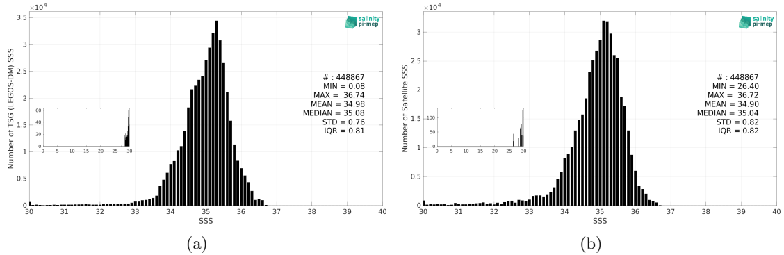
Figure 3: Histograms of SSS from TSG (LEGOS-DM) (a) and Aquarius SSS L3 OR v5 - 7-Day running - Rain mask (NASA-GSFC) (b) considering all match-up pairs per bins of 0.1 over the Pacific Ocean Pi-MEP region and for the full satellite product period.
