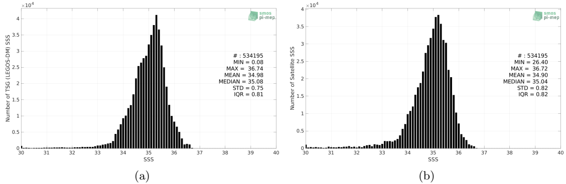
Figure 2: Histograms of SSS from TSG (LEGOS-DM) (a) and Aquarius SSS L3 OR v5 - 7-Day running - Rain masks (NASA-GSFC) (b) considering all match-up pairs per bins of 0.1 over the Pacific Ocean Pi-MEP region and for the full satellite product period.
