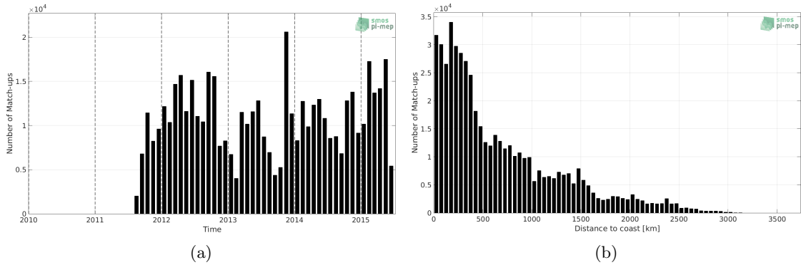
Figure 1: Number of match-ups between TSG-LEGOS-DM and Aquarius-L3-OR-V5-7DAY-RUNNING-RAIN-MASK-1DEG SSS as a function of time (a) and as function of the distance to coast (b) over the Pacific Ocean Pi-MEP region and for the full satellite product period.
