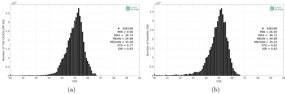
Figure 2: Histograms of SSS from TSG-LEGOS-DM (a) and Aquarius-L3-OR-V5-7DAY-RUNNING-RAIN-MASK-1DEG (b) considering all match-up pairs per bins of 0.1 over the Pacific Ocean Pi-MEP region and for the full satellite product period.
