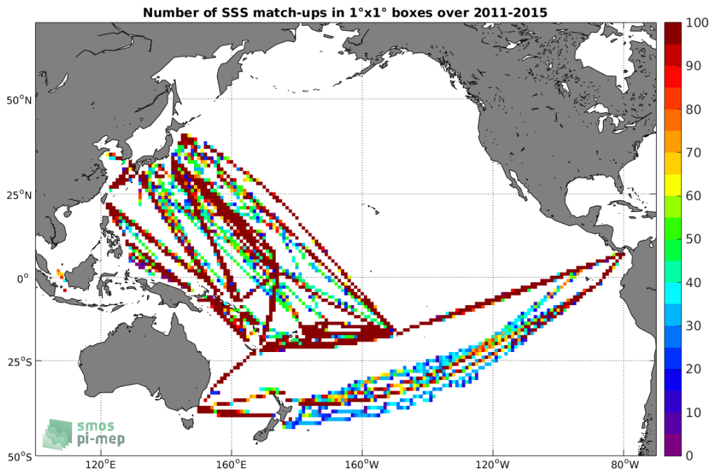
Figure 4: Number of SSS match-ups between TSG-LEGOS-DM SSS and the Aquarius-L3-OR-V5-7DAY-RUNNING-RAIN-MASK-1DEG SSS product for the Pacific Ocean Pi-MEP region over 1^\circ \times 1^\circ boxes and for the full satellite product period.
