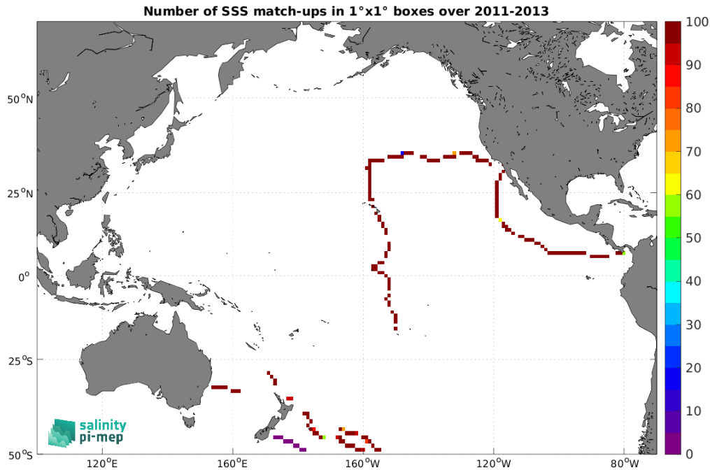
Figure 5: Number of SSS match-ups between TSG (GOSUD-Sailing-ship) SSS and the Aquarius SSS L3 OR v5 - 7-Day running - Rain mask (NASA-GSFC) SSS product for the Pacific Ocean Pi-MEP region over 1^\circ \times 1^\circ boxes and for the full satellite product period.
