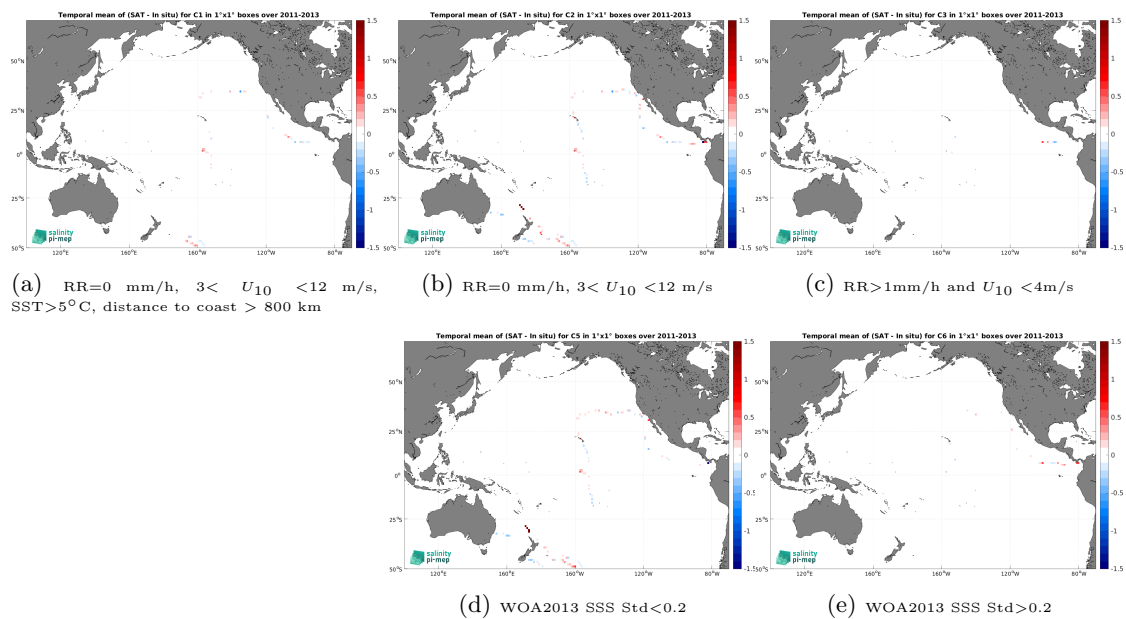
Figure 14: Temporal mean gridded over spatial boxes of size 1^\circ \times 1^\circ of \Delta SSS (Aquarius SSS L3 OR v5 - 7-Day running - Rain mask (NASA-GSFC) - TSG (GOSUD-Sailing-ship)) for 5 different subdatasets corresponding to:RR=0 mm/h, 3 < U_{10} < 12 m/s, SST >5^\circ\text{C} , distance to coast > 800 km (a), RR=0 mm/h, 3 < U_{10} < 12 m/s (b), RR >1 mm/h and U_{10} < 4 m/s (c), WOA2013 SSS Std <0.2 (d), WOA2013 SSS Std >0.2 (e).
