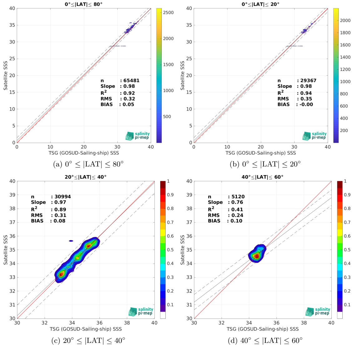
Figure 10: Contour maps of the concentration of Aquarius SSS L3 OR v5 - 7-Day running - Rain mask (NASA-GSFC) SSS (y-axis) versus TSG (GOSUD-Sailing-ship) SSS (x-axis) at match-up pairs for different latitude bands. For each plot, the red line shows x=y . The black thin and dashed lines indicate a linear fit through the data cloud and the \pm 95\% confidence levels, respectively. The number match-up pairs n , the slope and R^2 coefficient of the linear fit, the root mean square (RMS) and the mean bias between satellite and in situ data are indicated for each latitude band in each plots.
