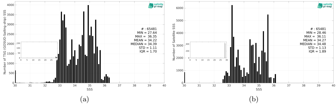
Figure 3: Histograms of SSS from TSG (GOSUD-Sailing-ship) (a) and Aquarius SSS L3 OR v5 - 7-Day running - Rain mask (NASA-GSFC) (b) considering all match-up pairs per bins of 0.1 over the Pacific Ocean Pi-MEP region and for the full satellite product period.
