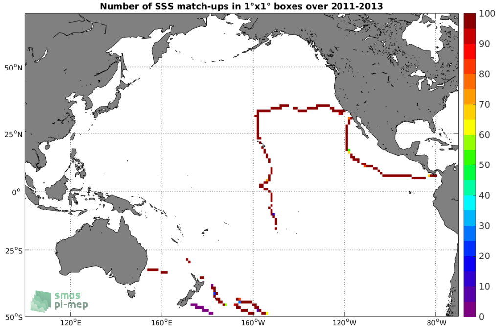
Figure 4: Number of SSS match-ups between TSG (GOSUD-Sailing-ship) SSS and the Aquarius SSS L3 OR v5 - 7-Day running - Rain mask (NASA-GSFC) SSS product for the Pacific Ocean Pi-MEP region over 1°x1° boxes and for the full satellite product period.
