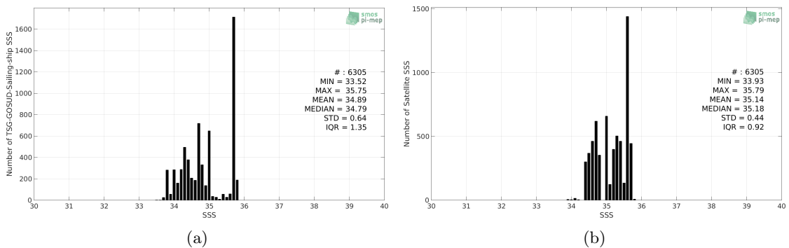
Figure 2: Histograms of SSS from TSG-GOSUD-Sailing-ship (a) and Aquarius-L3-OR-V5-7DAY-RUNNING-RAIN-MASK-1DEG (b) considering all match-up pairs per bins of 0.1 over the Pacific Ocean Pi-MEP region and for the full satellite product period.
