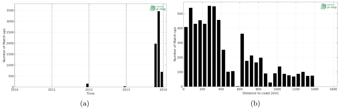
Figure 1: Number of match-ups between TSG-GOSUD-Sailing-ship and Aquarius-L3-OR-V5-7DAY-RUNNING-RAIN-MASK-1DEG SSS as a function of time (a) and as function of the distance to coast (b) over the Pacific Ocean Pi-MEP region and for the full satellite product period.
