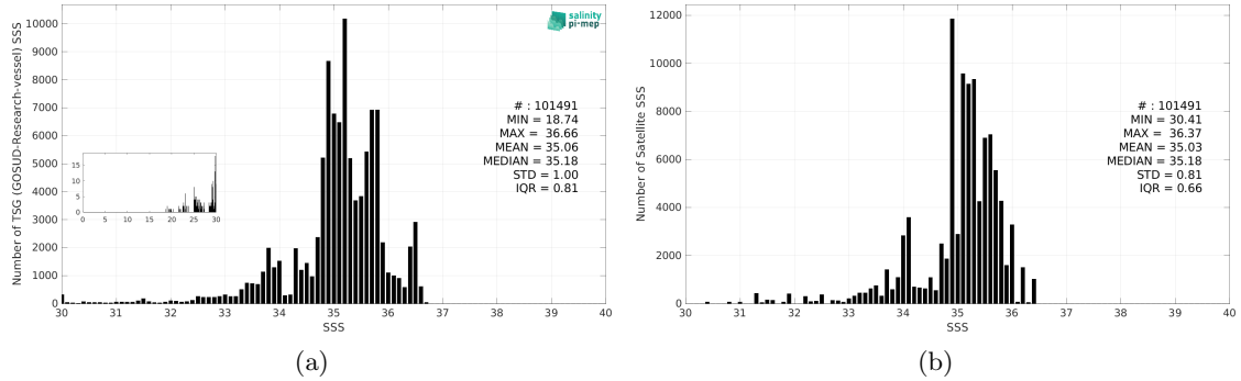
Figure 3: Histograms of SSS from TSG (GOSUD-Research-vessel) (a) and Aquarius SSS L3 OR v5 - 7-Day running - Rain mask (NASA-GSFC) (b) considering all match-up pairs per bins of 0.1 over the Pacific Ocean Pi-MEP region and for the full satellite product period.
