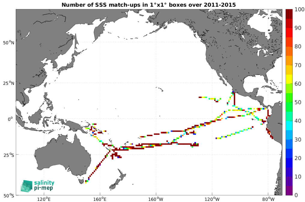
Figure 5: Number of SSS match-ups between TSG (GOSUD-Research-vessel) SSS and the Aquarius SSS L3 OR v5 - 7-Day running - Rain mask (NASA-GSFC) SSS product for the Pacific Ocean Pi-MEP region over 1^\circ \times 1^\circ boxes and for the full satellite product period.
