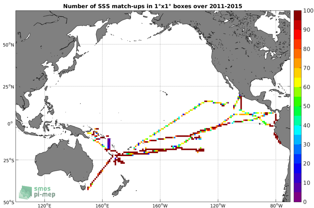
Figure 4: Number of SSS match-ups between TSG-GOSUD-Research-vessel SSS and the Aquarius-L3-OR-V5-7DAY-RUNNING-RAIN-MASK-1DEG SSS product for the Pacific Ocean Pi-MEP region over 1^{\circ} \times 1^{\circ} boxes and for the full satellite product period.
