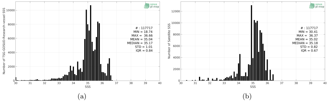
Figure 2: Histograms of SSS from TSG-GOSUD-Research-vessel (a) and Aquarius-L3-OR-V5-7DAY-RUNNING-RAIN-MASK-1DEG (b) considering all match-up pairs per bins of 0.1 over the Pacific Ocean Pi-MEP region and for the full satellite product period.
