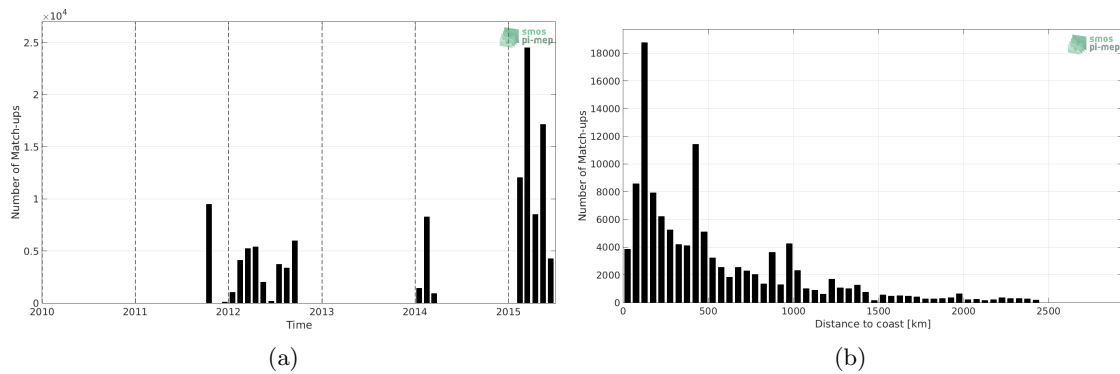
Figure 1: Number of match-ups between TSG-GOSUD-Research-vessel and Aquarius-L3-OR-V5-7DAY-RUNNING-RAIN-MASK-1DEG SSS as a function of time (a) and as function of the distance to coast (b) over the Pacific Ocean Pi-MEP region and for the full satellite product period.
