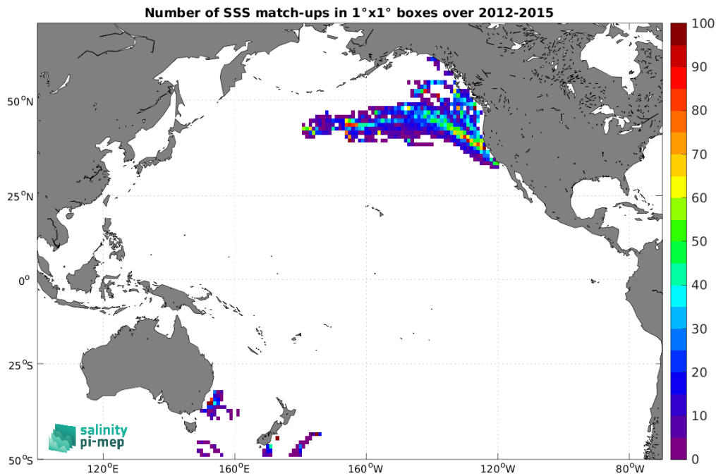
Figure 4: Number of SSS match-ups between Marine mammals SSS and the Aquarius SSS L3 OR v5 - 7-Day running - Rain mask (NASA-GSFC) SSS product for the Pacific Ocean Pi-MEP region over 1^\circ \times 1^\circ boxes and for the full satellite product period.
