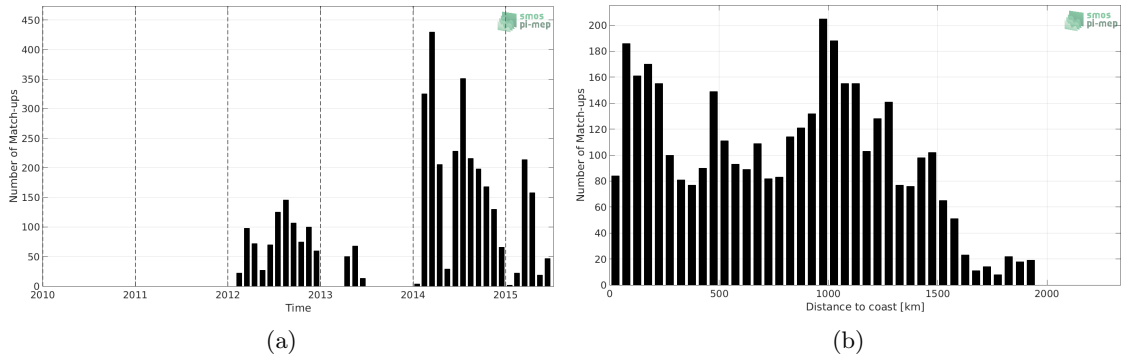
Figure 1: Number of match-ups between Sea mammals and Aquarius-L3-OR-V5-7DAY-RUNNING-RAIN-MASK-1DEG SSS as a function of time (a) and as function of the distance to coast (b) over the Pacific Ocean Pi-MEP region and for the full satellite product period.
