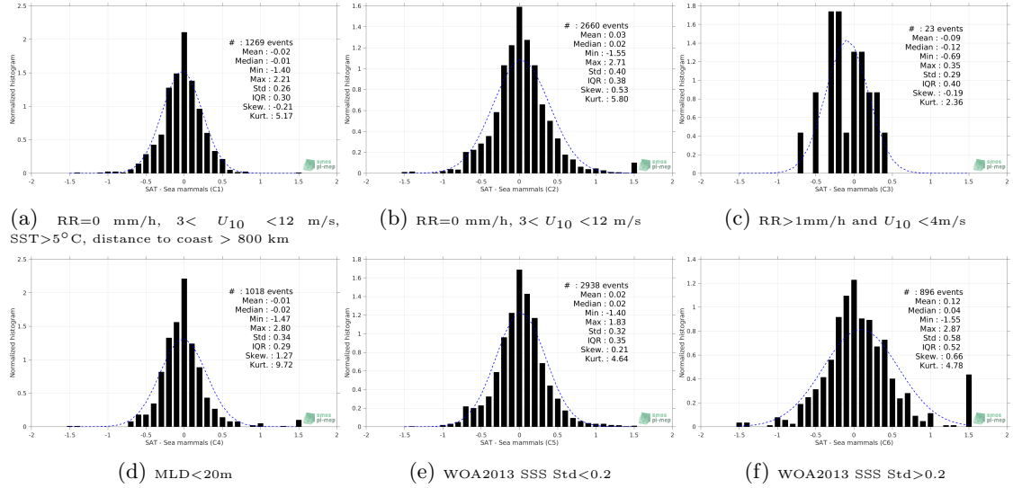
Figure 13: Normalized histogram of \Delta\text{SSS} (Aquarius-L3-OR-V5-7DAY-RUNNING-RAIN-MASK-1DEG - Sea mammals) for 6 different subdatasets corresponding to: RR=0 mm/h, 3 < U_{10} < 12 m/s, SST>5°C, distance to coast > 800 km (a), RR=0 mm/h, 3 < U_{10} < 12 m/s (b), RR>1mm/h and U_{10} < 4 m/s (c), MLD<20m (d), WOA2013 SSS Std<0.2 (e), WOA2013 SSS Std>0.2 (f).
