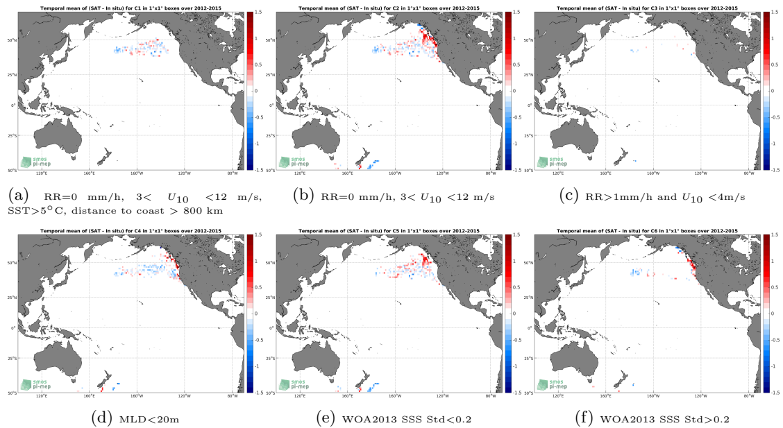
Figure 12: Temporal mean gridded over spatial boxes of size 1^\circ \times 1^\circ of \Delta SSS (Aquarius-L3-OR-V5-7DAY-RUNNING-RAIN-MASK-1DEG - Sea mammals) for 6 different subdatasets corresponding to:RR=0 mm/h, 3 < U_{10} < 12 m/s, SST >5^\circ C, distance to coast > 800 km (a), RR=0 mm/h, 3 < U_{10} < 12 m/s (b), RR >1 mm/h and U_{10} < 4 m/s (c),MLD <20 m (d),WOA2013 SSS Std <0.2 (e),WOA2013 SSS Std >0.2 (f).
