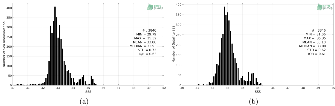
Figure 2: Histograms of SSS from Sea mammals (a) and Aquarius-L3-OR-V5-7DAY-RUNNING-RAIN-MASK-1DEG (b) considering all match-up pairs per bins of 0.1 over the Pacific Ocean Pi-MEP region and for the full satellite product period.
