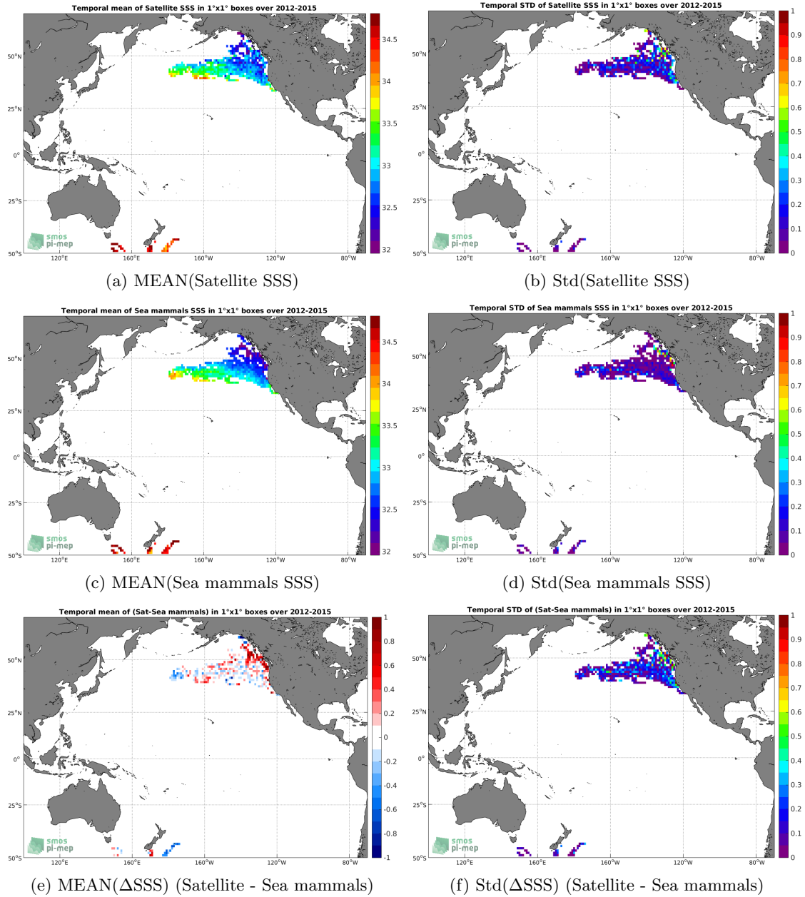
Figure 6: Temporal mean (left) and Std (right) of SSS from Aquarius-L3-OR-V5-7DAY-RUNNING-RAIN-MASK-1DEG (top), Sea mammals (middle), and of \Delta SSS (Satellite - Sea mammals). Only match-up pairs are used to generate these maps.
