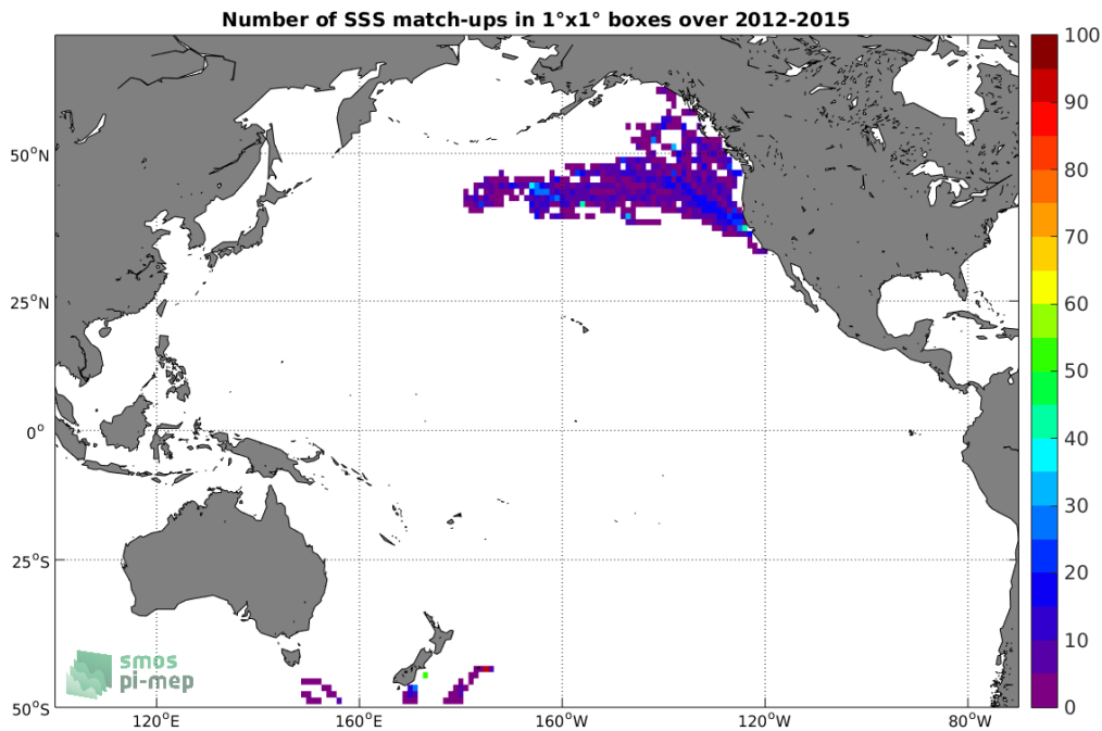
Figure 4: Number of SSS match-ups between Sea mammals SSS and the Aquarius-L3-OR-V5-7DAY-RUNNING-RAIN-MASK-1DEG SSS product for the Pacific Ocean Pi-MEP region over 1°x1° boxes and for the full satellite product period.
