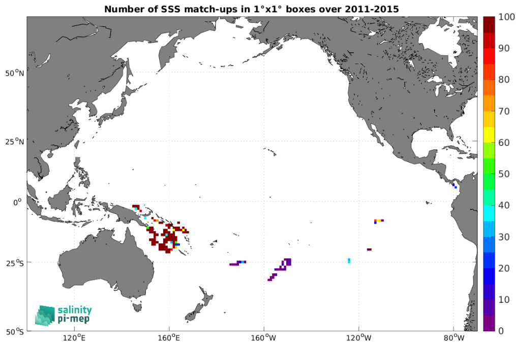
Figure 4: Number of SSS match-ups between Surface drifters SSS and the Aquarius SSS L3 OR v5 - 7-Day running - Rain mask (NASA-GSFC) SSS product for the Pacific Ocean Pi-MEP region over 1^\circ \times 1^\circ boxes and for the full satellite product period.
