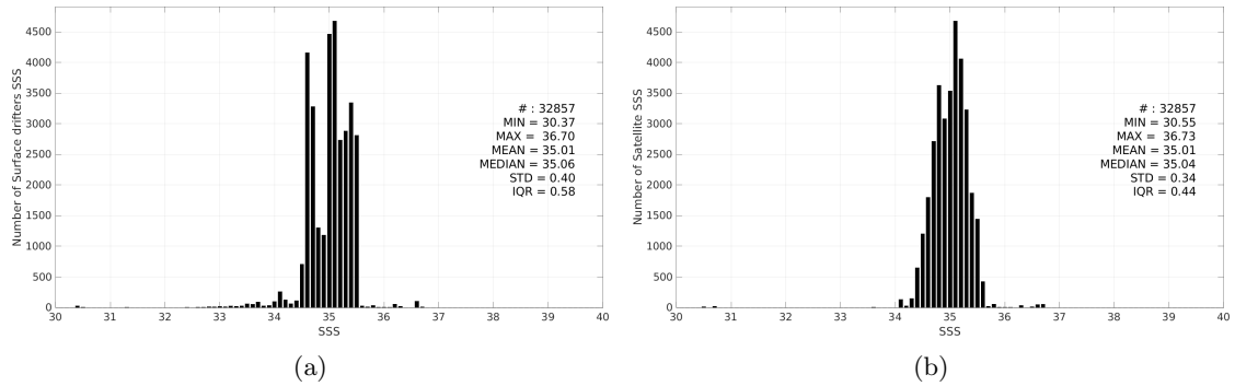
Figure 3: Histograms of SSS from Surface drifters (a) and Aquarius SSS L3 OR v5 - 7-Day running - Rain mask (NASA-GSFC) (b) considering all match-up pairs per bins of 0.1 over the Pacific Ocean Pi-MEP region and for the full satellite product period.
