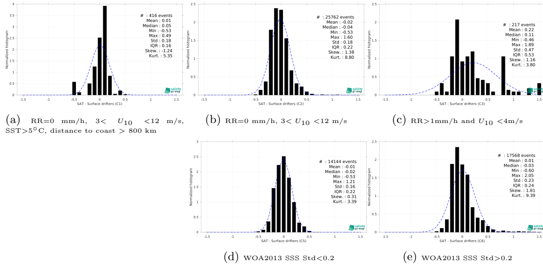
Figure 14: Normalized histogram of \Delta\text{SSS} (Aquarius SSS L3 OR v5 - 7-Day running - Rain mask (NASA-GSFC) - Surface drifters) for 5 different subdatasets corresponding to: RR=0 mm/h, 3 < U_{10} < 12 m/s, SST>5°C, distance to coast > 800 km (a), RR=0 mm/h, 3 < U_{10} < 12 m/s (b), RR>1mm/h and U_{10} < 4 m/s (c), WOA2013 SSS Std<0.2 (d), WOA2013 SSS Std>0.2 (e).
