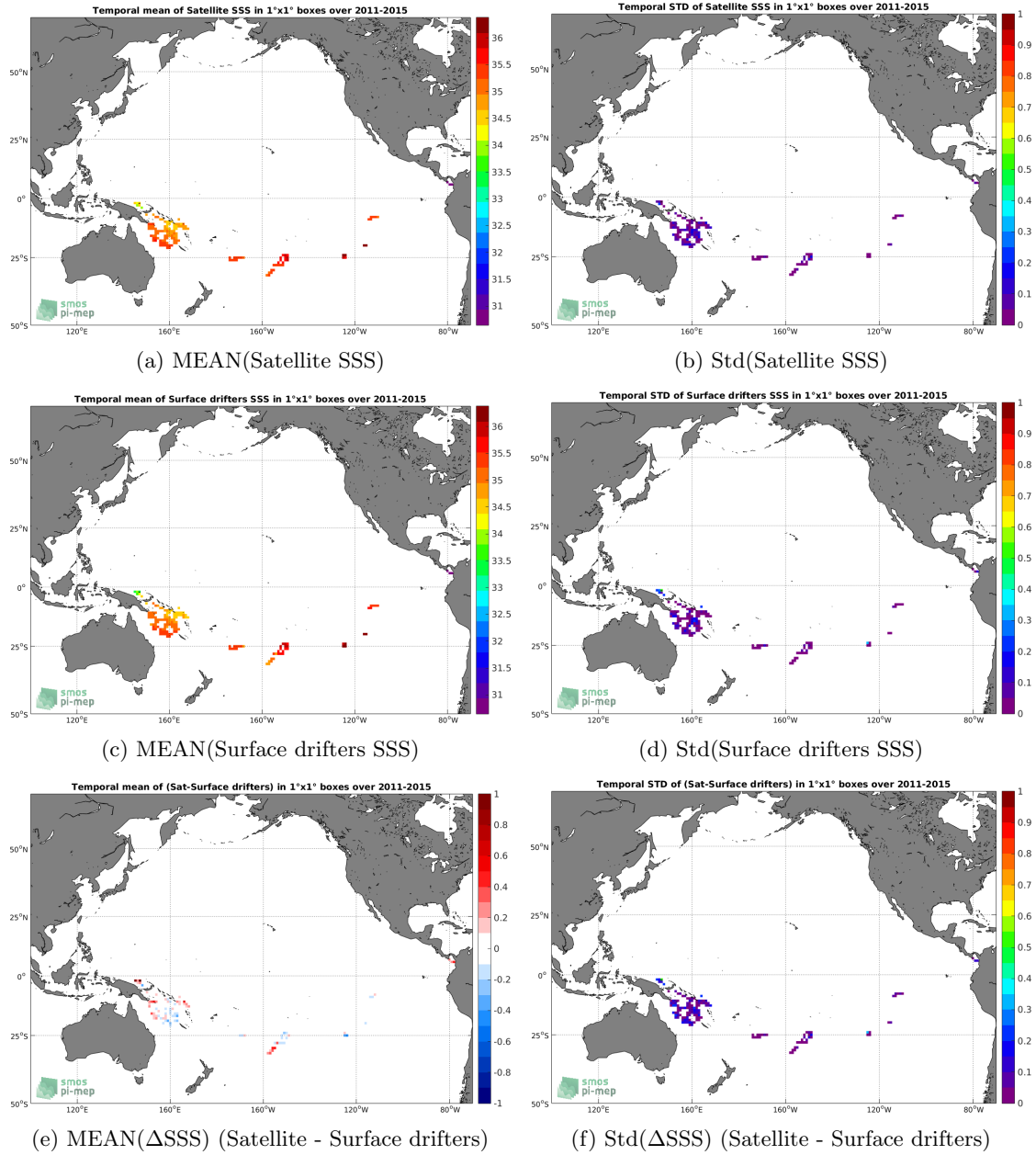
Figure 5: Temporal mean (left) and Std (right) of SSS from Aquarius-L3-OR-V5-7DAY-RUNNING-RAIN-MASK-1DEG (top), Surface drifters (middle), and of \Delta SSS (Satellite - Surface drifters). Only match-up pairs are used to generate these maps.
