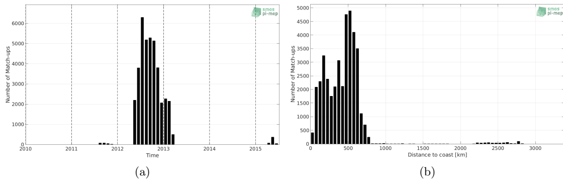
Figure 1: Number of match-ups between Surface drifters and Aquarius-L3-OR-V5-7DAY-RUNNING-RAIN-MASK-1DEG SSS as a function of time (a) and as function of the distance to coast (b) over the Pacific Ocean Pi-MEP region and for the full satellite product period.
