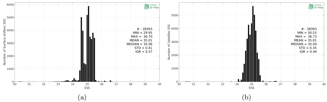
Figure 2: Histograms of SSS from Surface drifters (a) and Aquarius-L3-OR-V5-7DAY-RUNNING-RAIN-MASK-1DEG (b) considering all match-up pairs per bins of 0.1 over the Pacific Ocean Pi-MEP region and for the full satellite product period.
