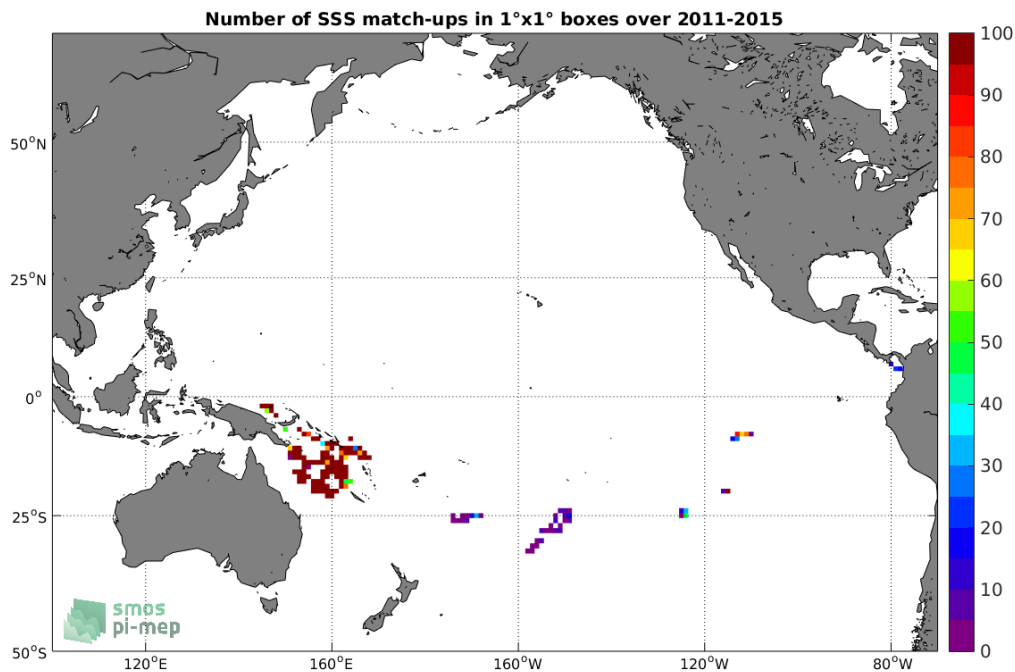
Figure 3: Number of SSS match-ups between Surface drifters SSS and the Aquarius-L3-OR-V5-7DAY-RUNNING-RAIN-MASK-1DEG SSS product for the Pacific Ocean Pi-MEP region over 1°x1° boxes and for the full satellite product period.
