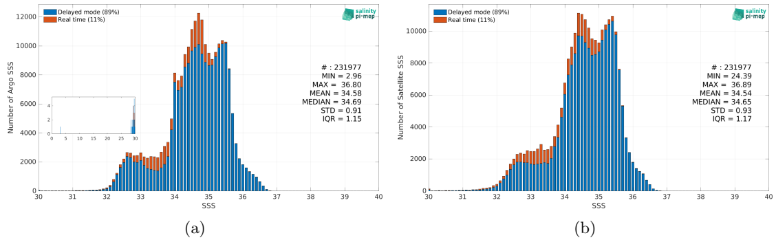
Figure 2: Histograms of SSS from Argo (a) and Aquarius SSS L3 OR v5 - 7-Day running - Rain mask (NASA-GSFC) (b) considering all match-up pairs per bins of 0.1 over the Pacific Ocean Pi-MEP region and for the full satellite product period.
