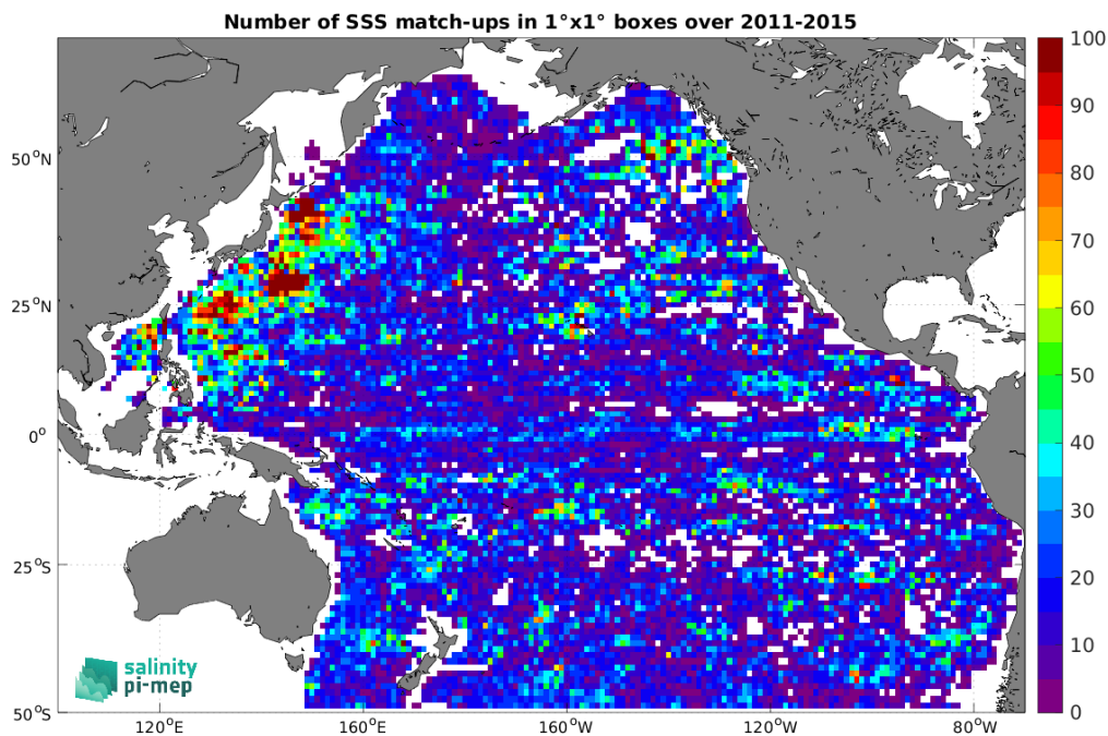
Figure 4: Number of SSS match-ups between Argo SSS and the Aquarius SSS L3 OR v5 - 7-Day running - Rain mask (NASA-GSFC) SSS product for the Pacific Ocean Pi-MEP region over 1^\circ \times 1^\circ boxes and for the full satellite product period.
