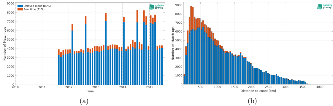
Figure 1: Number of match-ups between Argo and Aquarius SSS L3 OR v5 - 7-Day running - Rain mask (NASA-GSFC) SSS as a function of time (a) and as function of the distance to coast (b) over the Pacific Ocean Pi-MEP region and for the full satellite product period.
