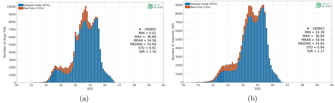
Figure 2: Histograms of SSS from Argo (a) and Aquarius SSS L3 OR v5 - 7-Day running - Rain mask (NASA-GSFC) (b) considering all match-up pairs per bins of 0.1 over the Pacific Ocean Pi-MEP region and for the full satellite product period.
