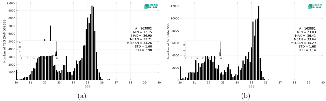
Figure 3: Histograms of SSS from TSG (SAMOS) (a) and Aquarius SSS L3 OR v5 - Monthly (NASA-GSFC) (b) considering all match-up pairs per bins of 0.1 over the Pacific Ocean Pi-MEP region and for the full satellite product period.
