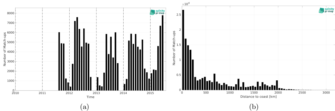
Figure 2: Number of match-ups between TSG (SAMOS) and Aquarius SSS L3 OR v5 - Monthly (NASA-GSFC) SSS as a function of time (a) and as function of the distance to coast (b) over the Pacific Ocean Pi-MEP region and for the full satellite product period.
