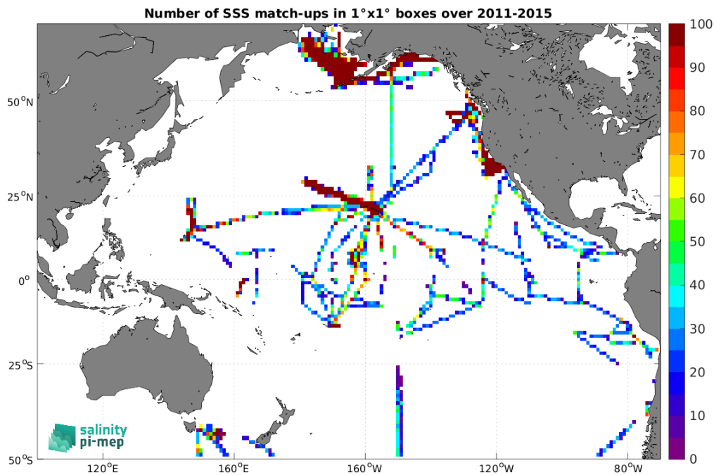
Figure 5: Number of SSS match-ups between TSG (SAMOS) SSS and the Aquarius SSS L3 OR v5 - Monthly (NASA-GSFC) SSS product for the Pacific Ocean Pi-MEP region over 1^\circ \times 1^\circ boxes and for the full satellite product period.
