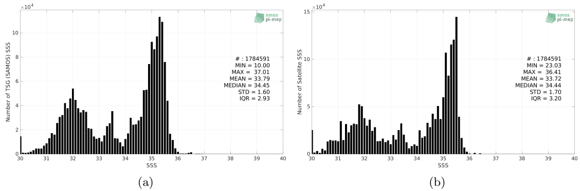
Figure 2: Histograms of SSS from TSG (SAMOS) (a) and Aquarius SSS L3 OR v5 - Monthly (NASA-GSFC) (b) considering all match-up pairs per bins of 0.1 over the Pacific Ocean Pi-MEP region and for the full satellite product period.
