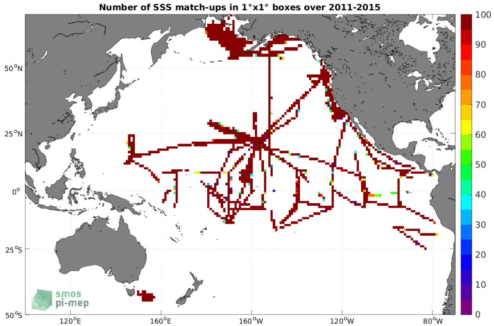
Figure 4: Number of SSS match-ups between TSG (SAMOS) SSS and the Aquarius SSS L3 OR v5 - Monthly (NASA-GSFC) SSS product for the Pacific Ocean Pi-MEP region over 1^\circ \times 1^\circ boxes and for the full satellite product period.
