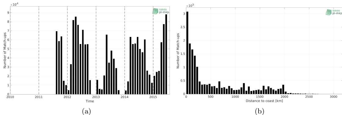
Figure 1: Number of match-ups between TSG (SAMOS) and Aquarius SSS L3 OR v5 - Monthly (NASA-GSFC) SSS as a function of time (a) and as function of the distance to coast (b) over the Pacific Ocean Pi-MEP region and for the full satellite product period.
