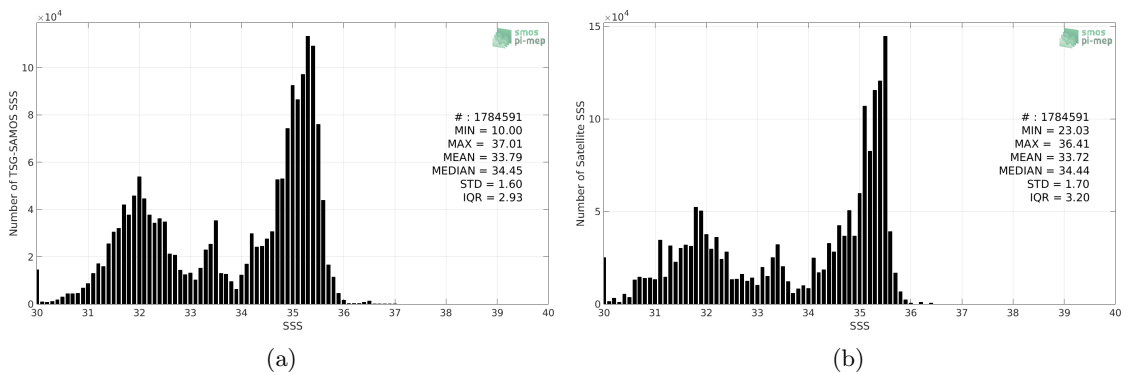
Figure 2: Histograms of SSS from TSG-SAMOS (a) and Aquarius-L3-OR-V5-MONTHLY-1DEG (b) considering all match-up pairs per bins of 0.1 over the Pacific Ocean Pi-MEP region and for the full satellite product period.
