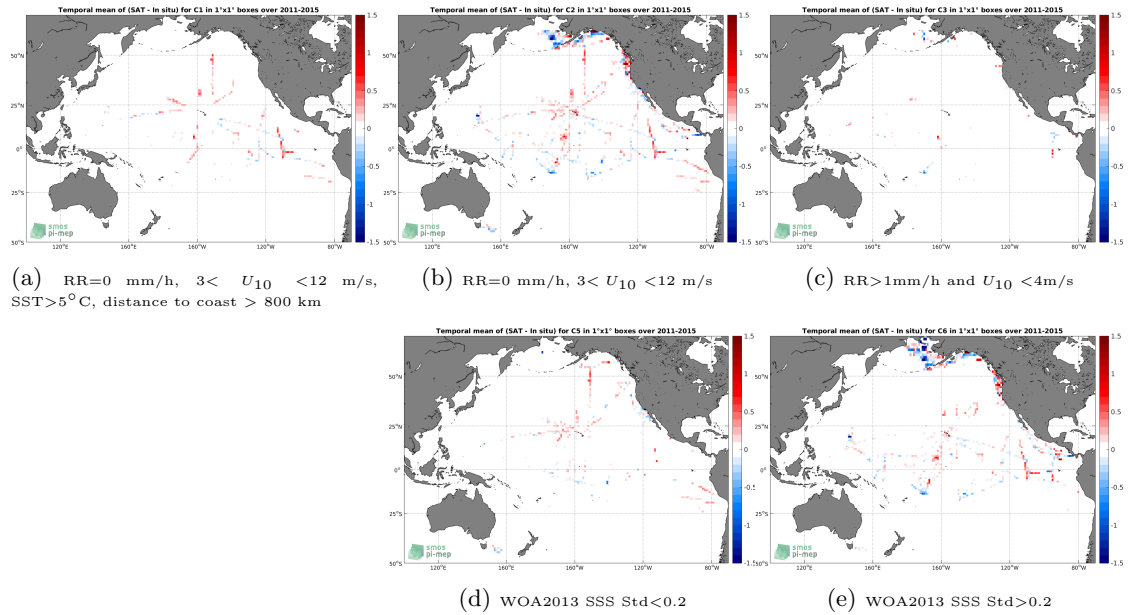
Figure 12: Temporal mean gridded over spatial boxes of size 1^\circ \times 1^\circ of \Delta SSS (Aquarius-L3-OR-V5-MONTHLY-1DEG - TSG-SAMOS) for 5 different subdatasets corresponding to:RR=0 mm/h, 3 < U_{10} < 12 m/s, SST > 5^\circ\text{C} , distance to coast > 800 km (a), RR=0 mm/h, 3 < U_{10} < 12 m/s (b), RR > 1 mm/h and U_{10} < 4 m/s (c), WOA2013 SSS Std < 0.2 (d), WOA2013 SSS Std > 0.2 (e).
