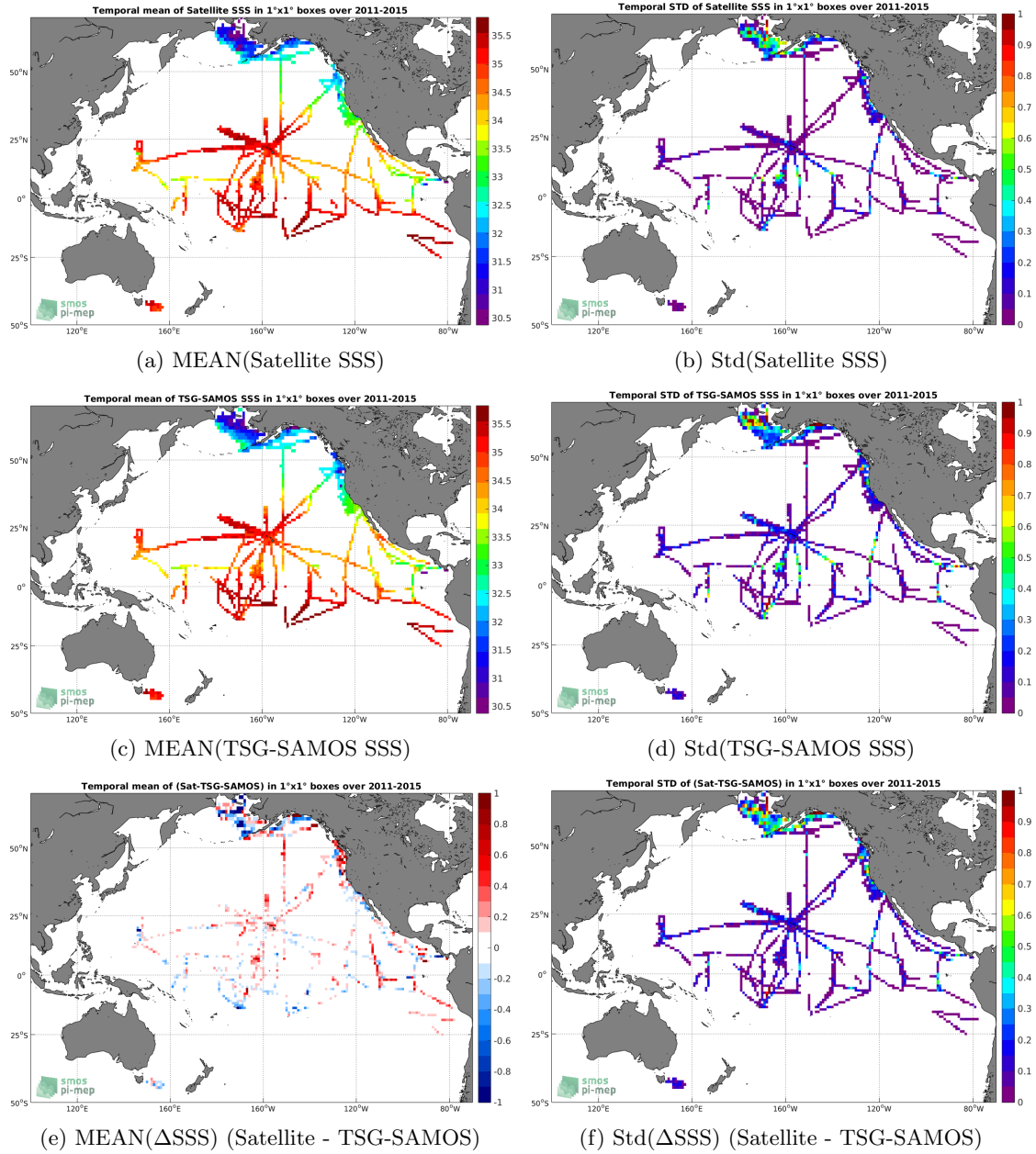
Figure 6: Temporal mean (left) and Std (right) of SSS from Aquarius-L3-OR-V5-MONTHLY-1DEG (top), TSG-SAMOS (middle), and of \Delta SSS (Satellite - TSG-SAMOS). Only match-up pairs are used to generate these maps.
