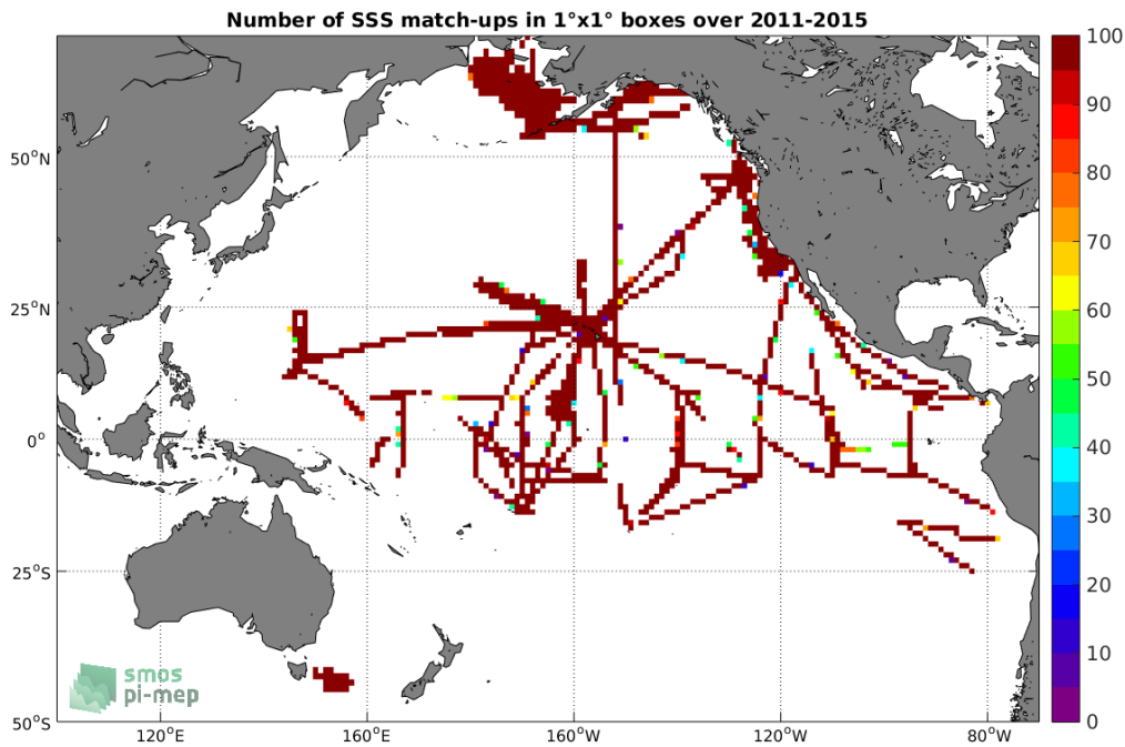
Figure 4: Number of SSS match-ups between TSG-SAMOS SSS and the Aquarius-L3-OR-V5-MONTHLY-1DEG SSS product for the Pacific Ocean Pi-MEP region over 1^\circ \times 1^\circ boxes and for the full satellite product period.
