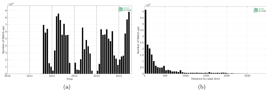
Figure 1: Number of match-ups between TSG-SAMOS and Aquarius-L3-OR-V5-MONTHLY-1DEG SSS as a function of time (a) and as function of the distance to coast (b) over the Pacific Ocean Pi-MEP region and for the full satellite product period.
