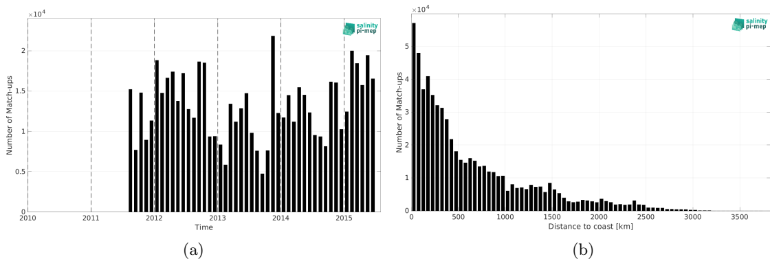
Figure 1: Number of match-ups between TSG (LEGOS-DM) and Aquarius SSS L3 OR v5 - Monthly (NASA-GSFC) SSS as a function of time (a) and as function of the distance to coast (b) over the Pacific Ocean Pi-MEP region and for the full satellite product period.
