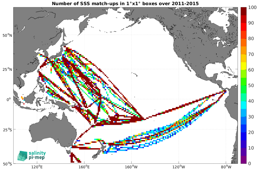
Figure 4: Number of SSS match-ups between TSG (LEGOS-DM) SSS and the Aquarius SSS L3 OR v5 - Monthly (NASA-GSFC) SSS product for the Pacific Ocean Pi-MEP region over 1^\circ \times 1^\circ boxes and for the full satellite product period.
