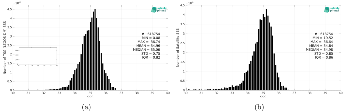
Figure 2: Histograms of SSS from TSG (LEGOS-DM) (a) and Aquarius SSS L3 OR v5 - Monthly (NASA-GSFC) (b) considering all match-up pairs per bins of 0.1 over the Pacific Ocean Pi-MEP region and for the full satellite product period.
