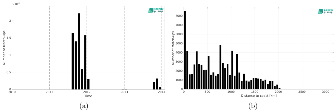
Figure 2: Number of match-ups between TSG (GOSUD-Sailing-ship) and Aquarius SSS L3 OR v5 - Monthly (NASA-GSFC) SSS as a function of time (a) and as function of the distance to coast (b) over the Pacific Ocean Pi-MEP region and for the full satellite product period.
