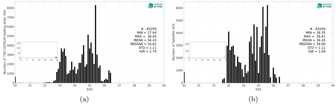
Figure 3: Histograms of SSS from TSG (GOSUD-Sailing-ship) (a) and Aquarius SSS L3 OR v5 - Monthly (NASA-GSFC) (b) considering all match-up pairs per bins of 0.1 over the Pacific Ocean Pi-MEP region and for the full satellite product period.
