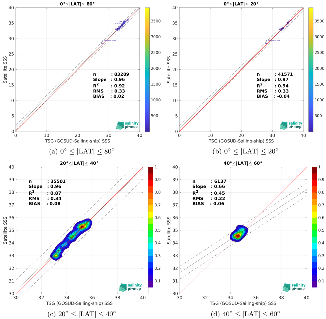
Figure 10: Contour maps of the concentration of Aquarius SSS L3 OR v5 - Monthly (NASA-GSFC) SSS (y-axis) versus TSG (GOSUD-Sailing-ship) SSS (x-axis) at match-up pairs for different latitude bands. For each plot, the red line shows x=y . The black thin and dashed lines indicate a linear fit through the data cloud and the \pm 95\% confidence levels, respectively. The number match-up pairs n , the slope and R^2 coefficient of the linear fit, the root mean square (RMS) and the mean bias between satellite and in situ data are indicated for each latitude band in each plots.
