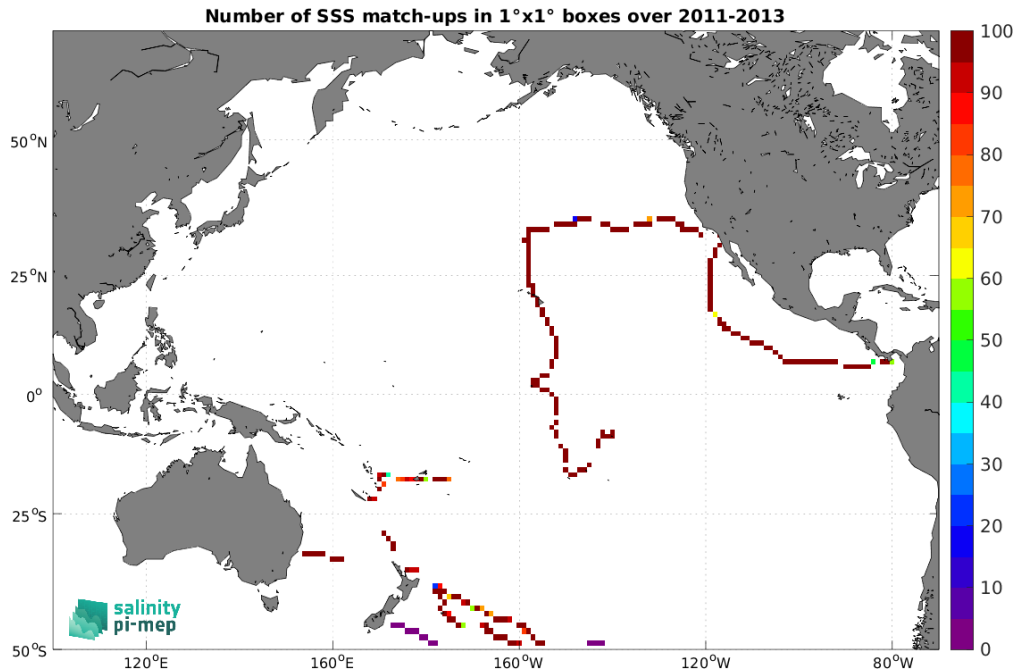
Figure 5: Number of SSS match-ups between TSG (GOSUD-Sailing-ship) SSS and the Aquarius SSS L3 OR v5 - Monthly (NASA-GSFC) SSS product for the Pacific Ocean Pi-MEP region over 1^\circ \times 1^\circ boxes and for the full satellite product period.
