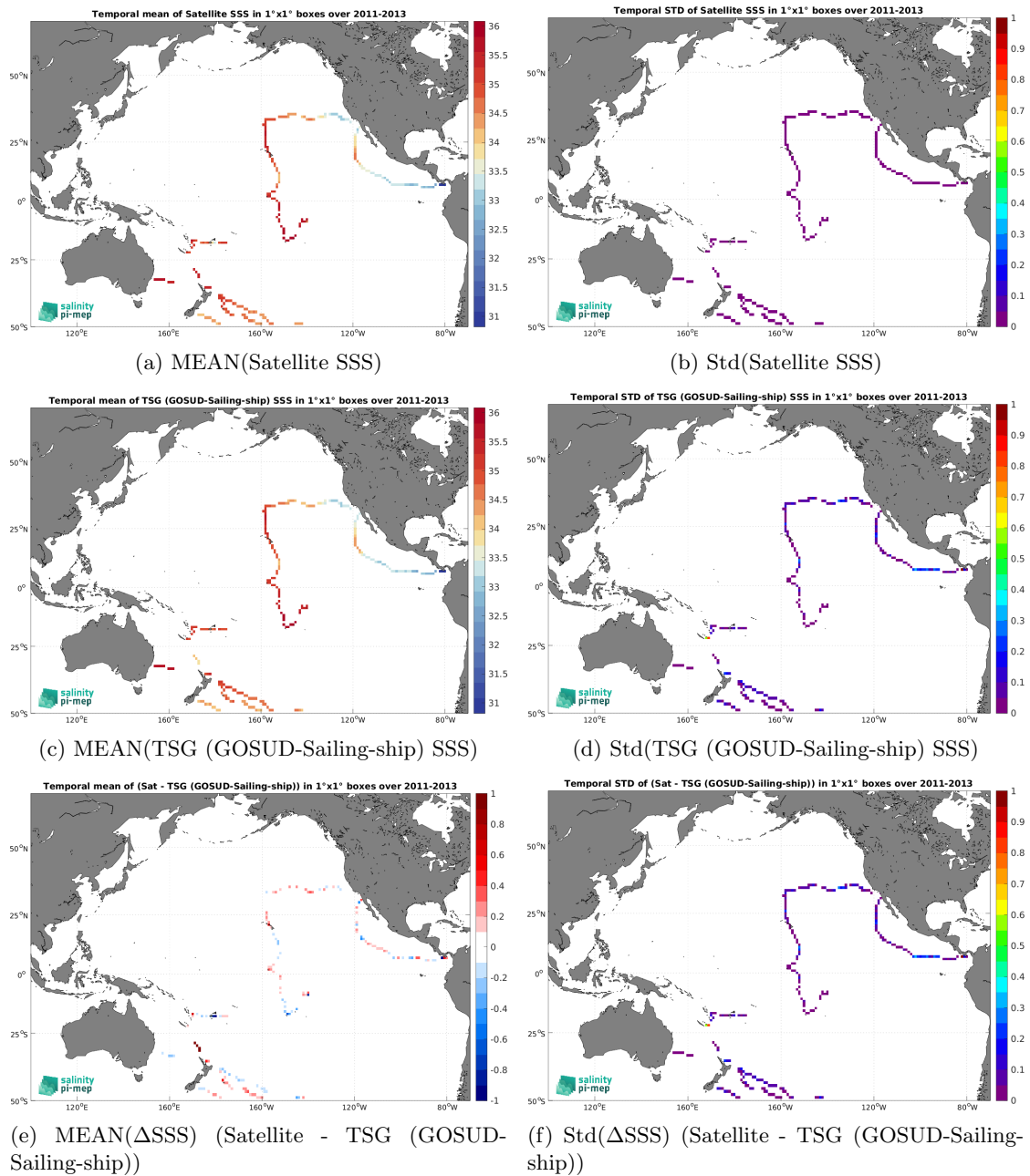
Figure 7: Temporal mean (left) and Std (right) of SSS from Aquarius SSS L3 OR v5 - Monthly (NASA-GSFC) (top), TSG (GOSUD-Sailing-ship) (middle), and of \Delta SSS (Satellite - TSG (GOSUD-Sailing-ship)). Only match-up pairs are used to generate these maps.
