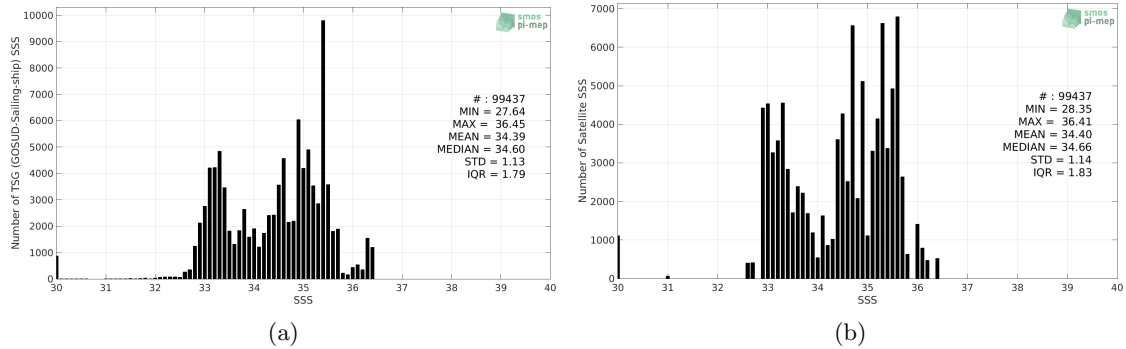
Figure 2: Histograms of SSS from TSG (GOSUD-Sailing-ship) (a) and Aquarius SSS L3 OR v5 - Monthly (NASA-GSFC) (b) considering all match-up pairs per bins of 0.1 over the Pacific Ocean Pi-MEP region and for the full satellite product period.
