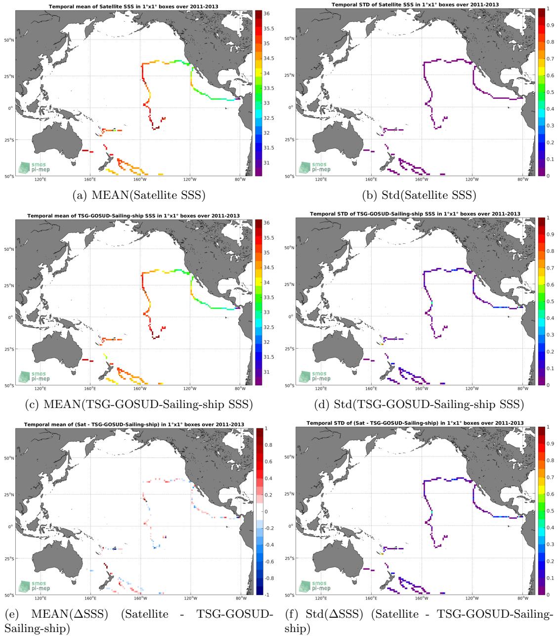
Figure 6: Temporal mean (left) and Std (right) of SSS from Aquarius-L3-OR-V5-MONTHLY-1DEG (top), TSG-GOSUD-Sailing-ship (middle), and of \Delta SSS (Satellite - TSG-GOSUD-Sailing-ship). Only match-up pairs are used to generate these maps.
