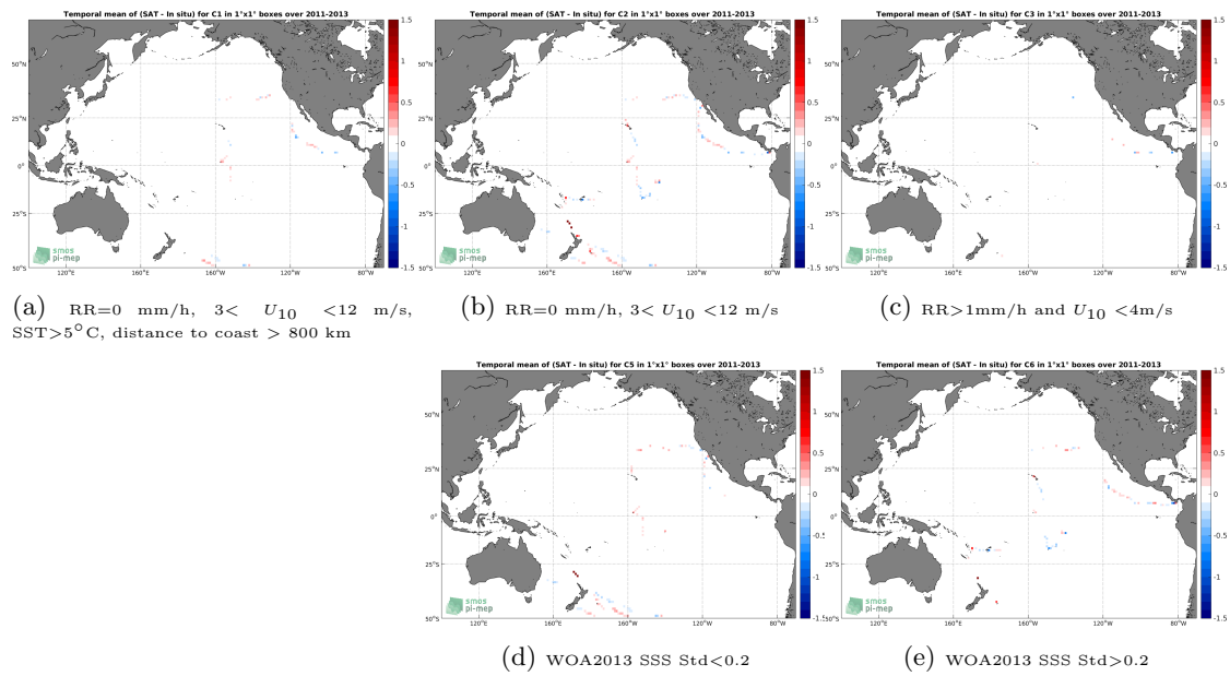
Figure 12: Temporal mean gridded over spatial boxes of size 1^\circ \times 1^\circ of \Delta SSS (Aquarius-L3-OR-V5-MONTHLY-1DEG - TSG-GOSUD-Sailing-ship) for 5 different subdatasets corresponding to: RR=0 mm/h, 3 < U_{10} < 12 m/s, SST > 5^\circ C , distance to coast > 800 km (a), RR=0 mm/h, 3 < U_{10} < 12 m/s (b), RR > 1 mm/h and U_{10} < 4 m/s (c), WOA2013 SSS Std < 0.2 (d), WOA2013 SSS Std > 0.2 (e).
