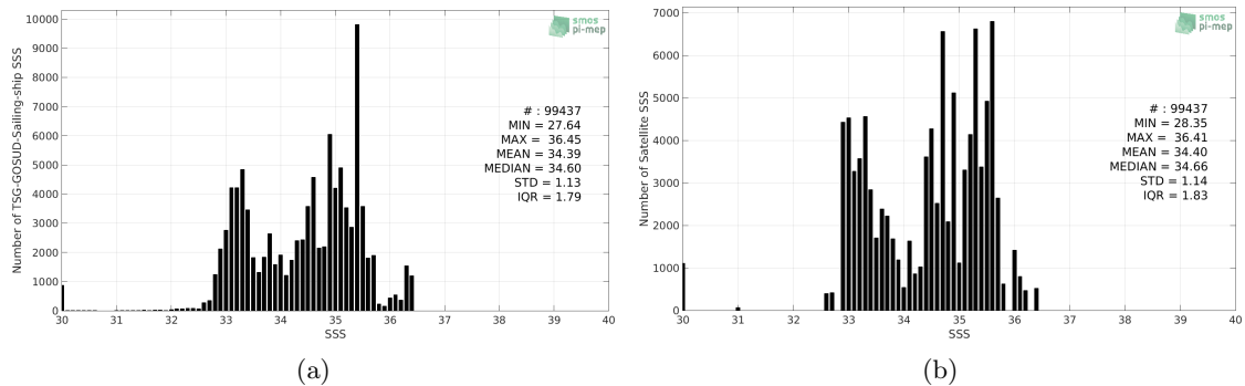
Figure 2: Histograms of SSS from TSG-GOSUD-Sailing-ship (a) and Aquarius-L3-OR-V5-MONTHLY-1DEG (b) considering all match-up pairs per bins of 0.1 over the Pacific Ocean Pi-MEP region and for the full satellite product period.
