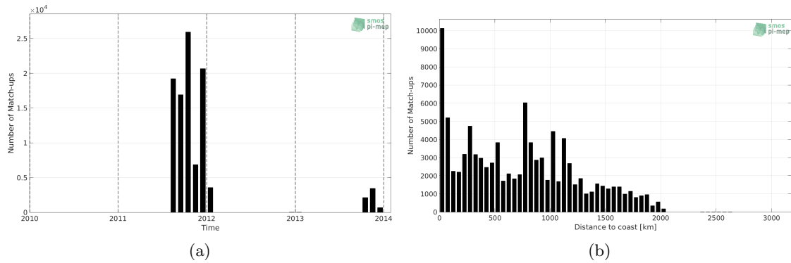
Figure 1: Number of match-ups between TSG-GOSUD-Sailing-ship and Aquarius-L3-OR-V5-MONTHLY-1DEG SSS as a function of time (a) and as function of the distance to coast (b) over the Pacific Ocean Pi-MEP region and for the full satellite product period.
