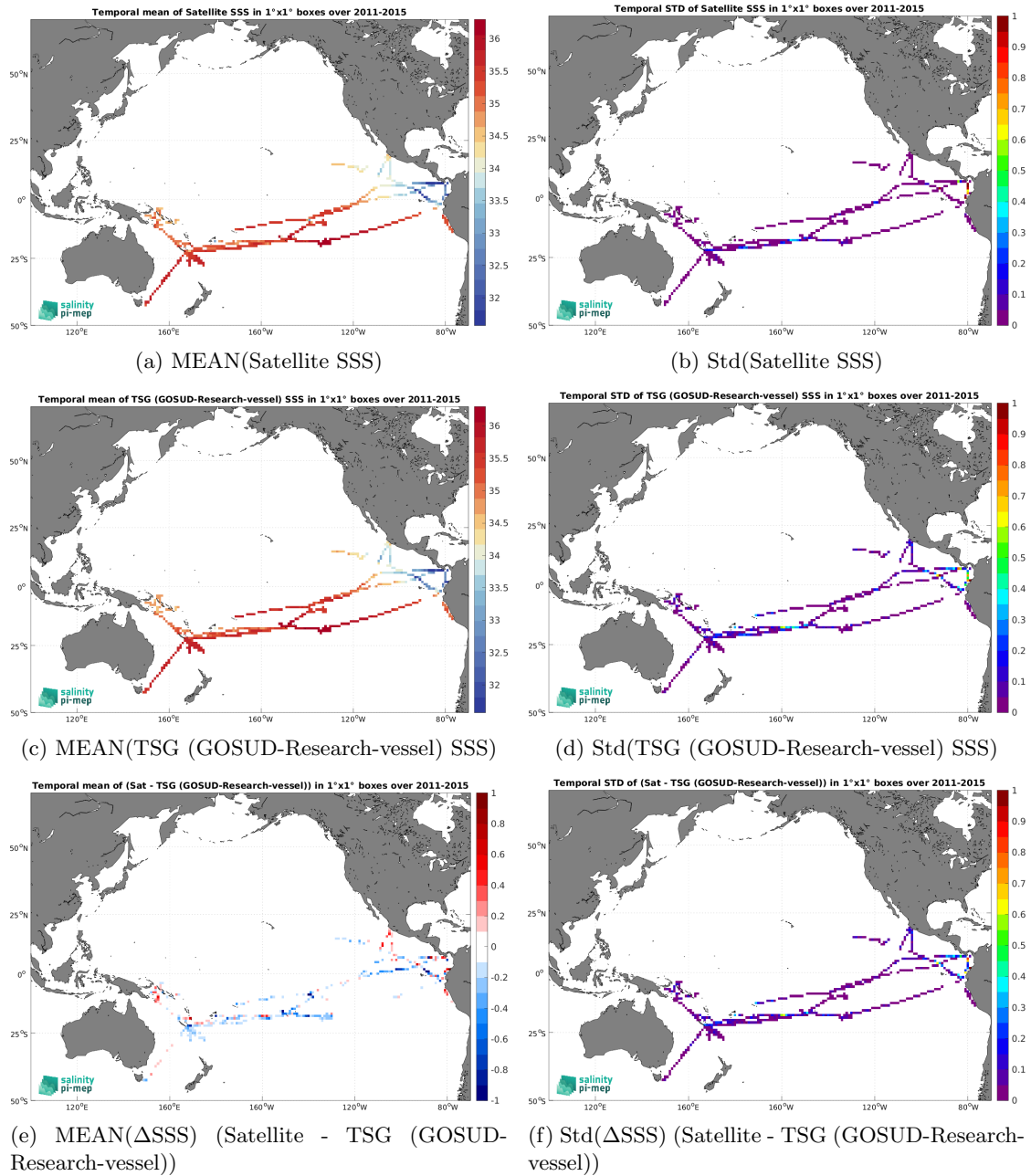
Figure 7: Temporal mean (left) and Std (right) of SSS from Aquarius SSS L3 OR v5 - Monthly (NASA-GSFC) (top), TSG (GOSUD-Research-vessel) (middle), and of \Delta SSS (Satellite - TSG (GOSUD-Research-vessel)). Only match-up pairs are used to generate these maps.
