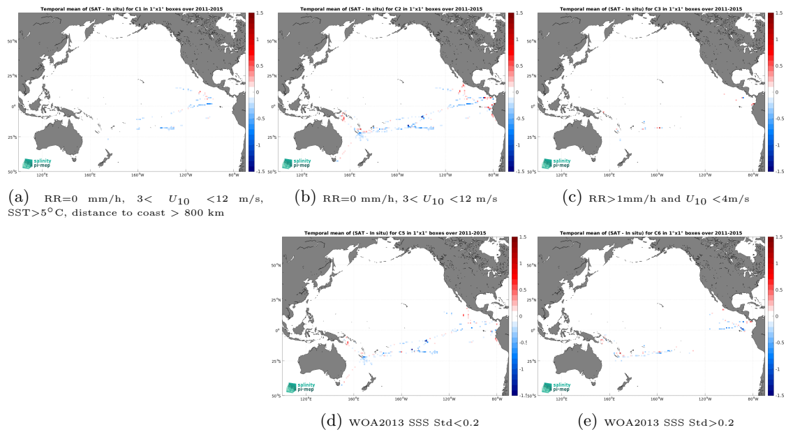
Figure 14: Temporal mean gridded over spatial boxes of size 1^\circ \times 1^\circ of \Delta SSS (Aquarius SSS L3 OR v5 - Monthly (NASA-GSFC) - TSG (GOSUD-Research-vessel)) for 5 different subdatasets corresponding to:RR=0 mm/h, 3 < U_{10} < 12 m/s, SST >5^\circ\text{C} , distance to coast > 800 km (a), RR=0 mm/h, 3 < U_{10} < 12 m/s (b), RR >1 mm/h and U_{10} < 4 m/s (c), WOA2013 SSS Std <0.2 (d), WOA2013 SSS Std >0.2 (e).
