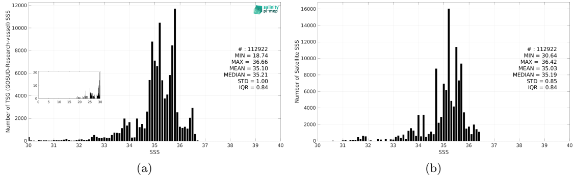
Figure 3: Histograms of SSS from TSG (GOSUD-Research-vessel) (a) and Aquarius SSS L3 OR v5 - Monthly (NASA-GSFC) (b) considering all match-up pairs per bins of 0.1 over the Pacific Ocean Pi-MEP region and for the full satellite product period.
