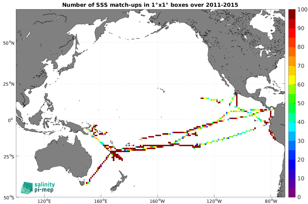
Figure 5: Number of SSS match-ups between TSG (GOSUD-Research-vessel) SSS and the Aquarius SSS L3 OR v5 - Monthly (NASA-GSFC) SSS product for the Pacific Ocean Pi-MEP region over 1^\circ \times 1^\circ boxes and for the full satellite product period.
