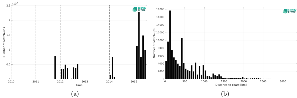
Figure 2: Number of match-ups between TSG (GOSUD-Research-vessel) and Aquarius SSS L3 OR v5 - Monthly (NASA-GSFC) SSS as a function of time (a) and as function of the distance to coast (b) over the Pacific Ocean Pi-MEP region and for the full satellite product period.
