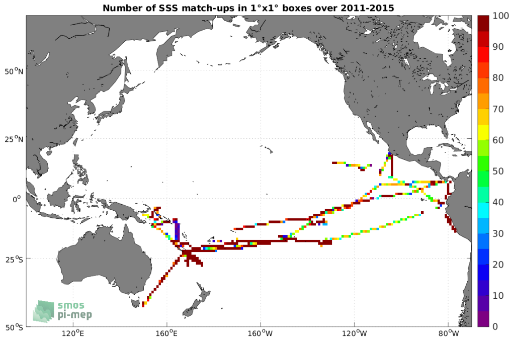
Figure 4: Number of SSS match-ups between TSG (GOSUD-Research-vessel) SSS and the Aquarius SSS L3 OR v5 - Monthly (NASA-GSFC) SSS product for the Pacific Ocean Pi-MEP region over 1^\circ \times 1^\circ boxes and for the full satellite product period.
