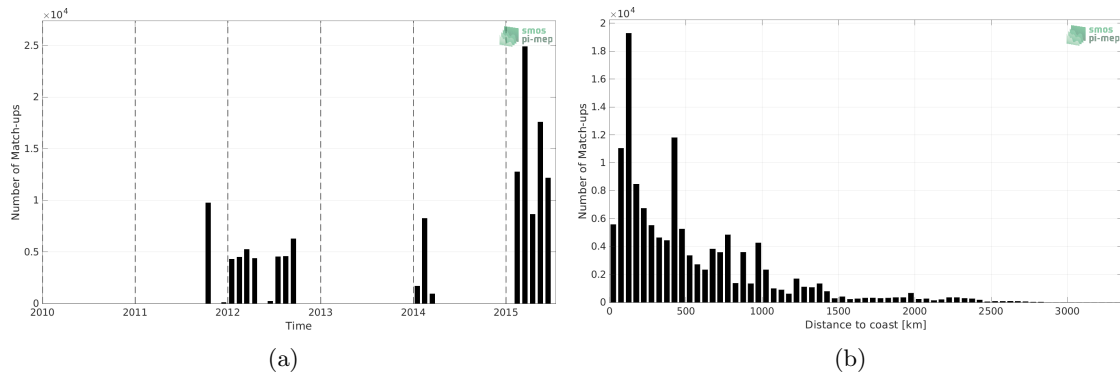
Figure 1: Number of match-ups between TSG (GOSUD-Research-vessel) and Aquarius SSS L3 OR v5 - Monthly (NASA-GSFC) SSS as a function of time (a) and as function of the distance to coast (b) over the Pacific Ocean Pi-MEP region and for the full satellite product period.
