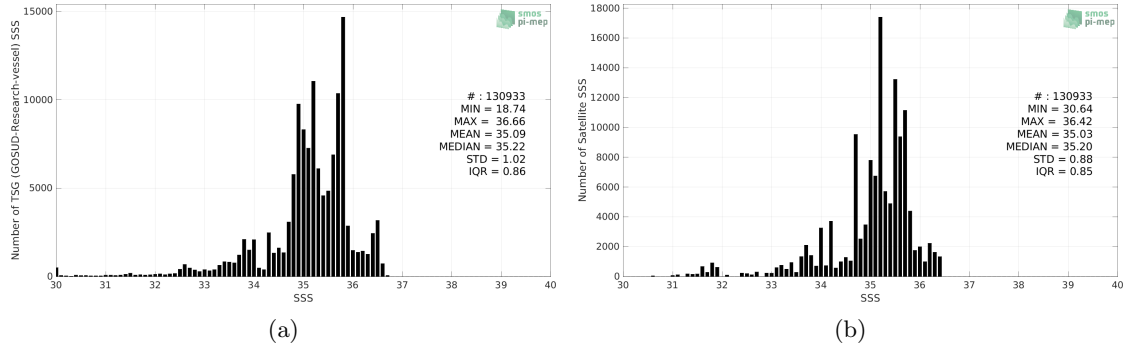
Figure 2: Histograms of SSS from TSG (GOSUD-Research-vessel) (a) and Aquarius SSS L3 OR v5 - Monthly (NASA-GSFC) (b) considering all match-up pairs per bins of 0.1 over the Pacific Ocean Pi-MEP region and for the full satellite product period.
