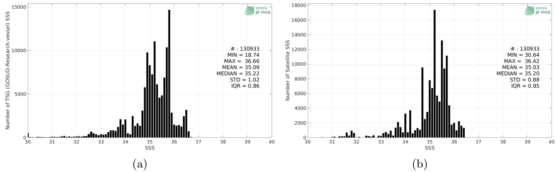
Figure 2: Histograms of SSS from TSG (GOSUD-Research-vessel) (a) and Aquarius SSS L3 OR v5 - Monthly (NASA-GSFC) (b) considering all match-up pairs per bins of 0.1 over the Pacific Ocean Pi-MEP region and for the full satellite product period.
