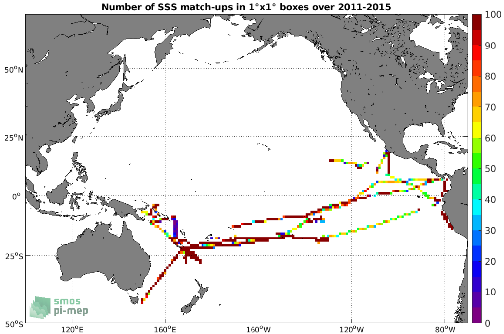
Figure 4: Number of SSS match-ups between TSG (GOSUD-Research-vessel) SSS and the Aquarius SSS L3 OR v5 - Monthly (NASA-GSFC) SSS product for the Pacific Ocean Pi-MEP region over 1°x1° boxes and for the full satellite product period.
