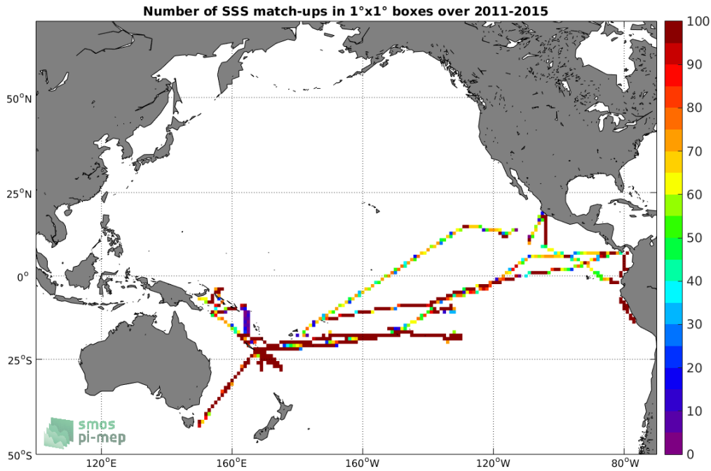
Figure 4: Number of SSS match-ups between TSG-GOSUD-Research-vessel SSS and the Aquarius-L3-OR-V5-MONTHLY-1DEG SSS product for the Pacific Ocean Pi-MEP region over 1^{\circ} \times 1^{\circ} boxes and for the full satellite product period.
