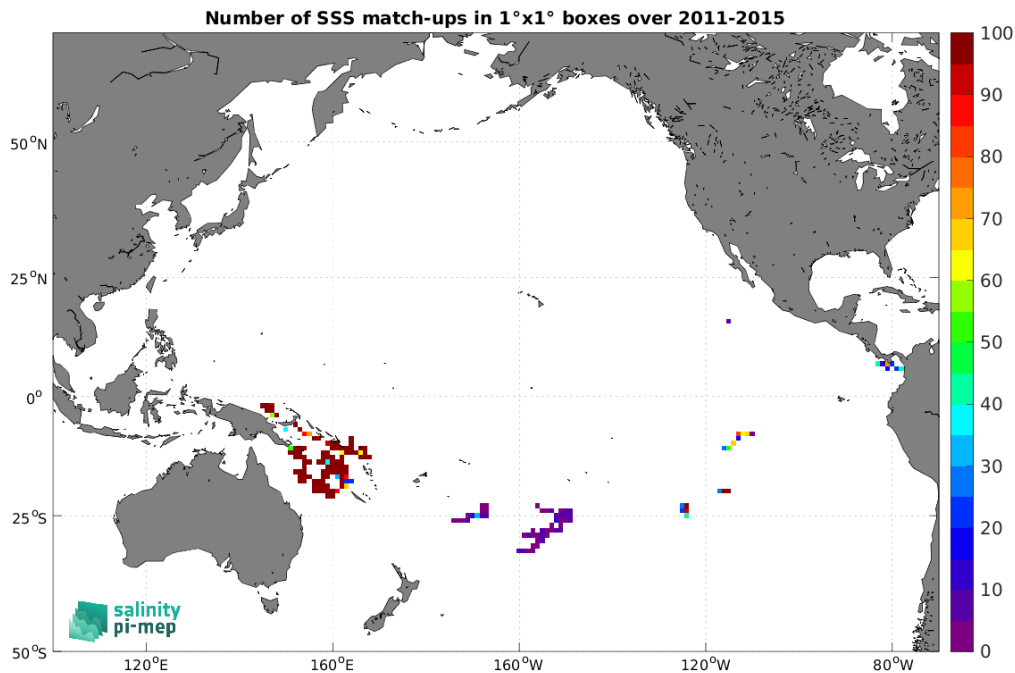
Figure 4: Number of SSS match-ups between Surface drifters SSS and the Aquarius SSS L3 OR v5 - Monthly (NASA-GSFC) SSS product for the Pacific Ocean Pi-MEP region over 1^\circ \times 1^\circ boxes and for the full satellite product period.
