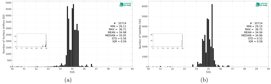
Figure 3: Histograms of SSS from Surface drifters (a) and Aquarius SSS L3 OR v5 - Monthly (NASA-GSFC) (b) considering all match-up pairs per bins of 0.1 over the Pacific Ocean Pi-MEP region and for the full satellite product period.
