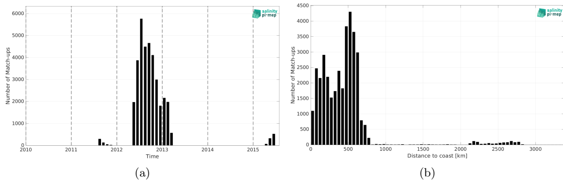
Figure 2: Number of match-ups between Surface drifters and Aquarius SSS L3 OR v5 - Monthly (NASA-GSFC) SSS as a function of time (a) and as function of the distance to coast (b) over the Pacific Ocean Pi-MEP region and for the full satellite product period.
