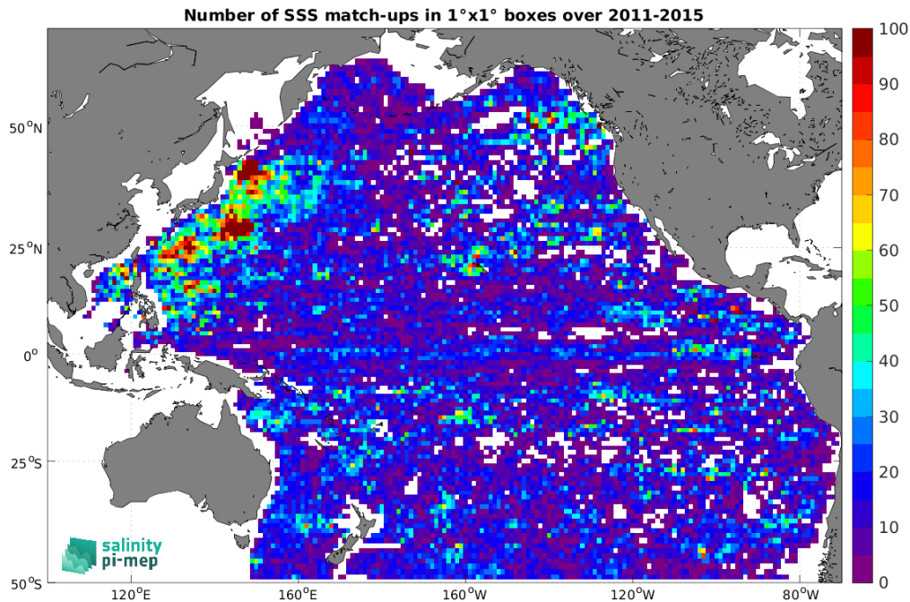
Figure 4: Number of SSS match-ups between Argo SSS and the Aquarius SSS L3 OR v5 - Monthly (NASA-GSFC) SSS product for the Pacific Ocean Pi-MEP region over 1^\circ \times 1^\circ boxes and for the full satellite product period.
