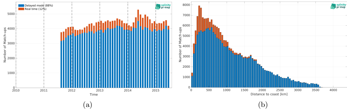
Figure 1: Number of match-ups between Argo and Aquarius SSS L3 OR v5 - Monthly (NASA-GSFC) SSS as a function of time (a) and as function of the distance to coast (b) over the Pacific Ocean Pi-MEP region and for the full satellite product period.
