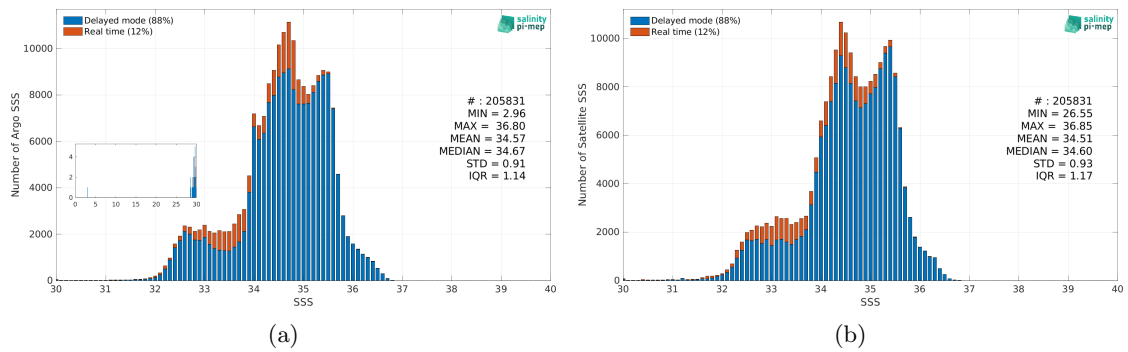
Figure 2: Histograms of SSS from Argo (a) and Aquarius SSS L3 OR v5 - Monthly (NASA-GSFC) (b) considering all match-up pairs per bins of 0.1 over the Pacific Ocean Pi-MEP region and for the full satellite product period.
