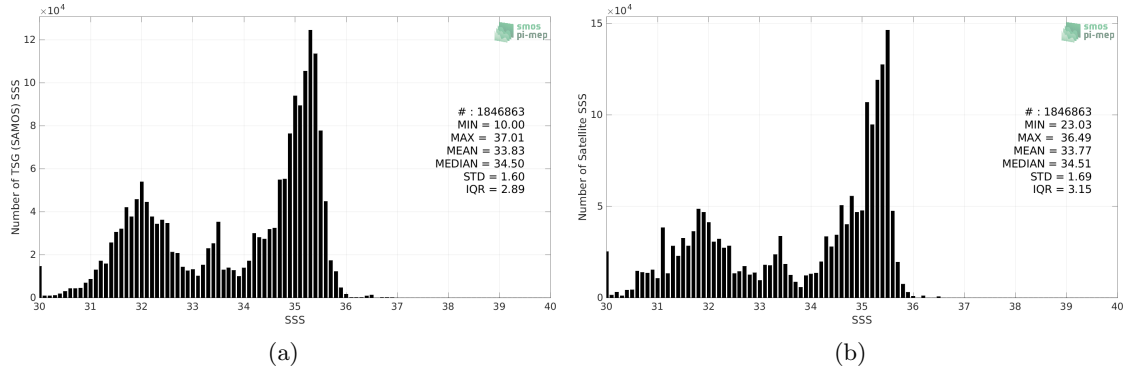
Figure 2: Histograms of SSS from TSG (SAMOS) (a) and Aquarius SSS L3 OR v5 - Monthly - Rain mask (NASA-GSFC) (b) considering all match-up pairs per bins of 0.1 over the Pacific Ocean Pi-MEP region and for the full satellite product period.
