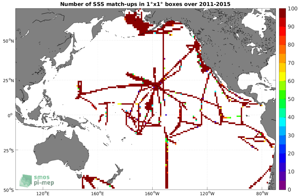
Figure 4: Number of SSS match-ups between TSG (SAMOS) SSS and the Aquarius SSS L3 OR v5 - Monthly - Rain mask (NASA-GSFC) SSS product for the Pacific Ocean Pi-MEP region over 1^\circ \times 1^\circ boxes and for the full satellite product period.
