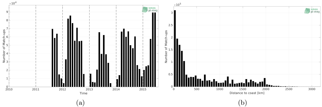
Figure 1: Number of match-ups between TSG (SAMOS) and Aquarius SSS L3 OR v5 - Monthly - Rain mask (NASA-GSFC) SSS as a function of time (a) and as function of the distance to coast (b) over the Pacific Ocean Pi-MEP region and for the full satellite product period.
