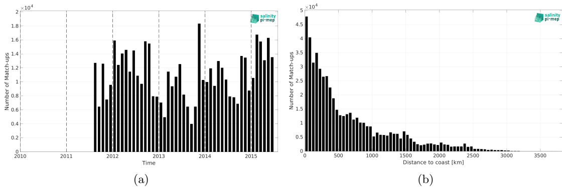
Figure 2: Number of match-ups between TSG (LEGOS-DM) and Aquarius SSS L3 OR v5 - Monthly - Rain mask (NASA-GSFC) SSS as a function of time (a) and as function of the distance to coast (b) over the Pacific Ocean Pi-MEP region and for the full satellite product period.
