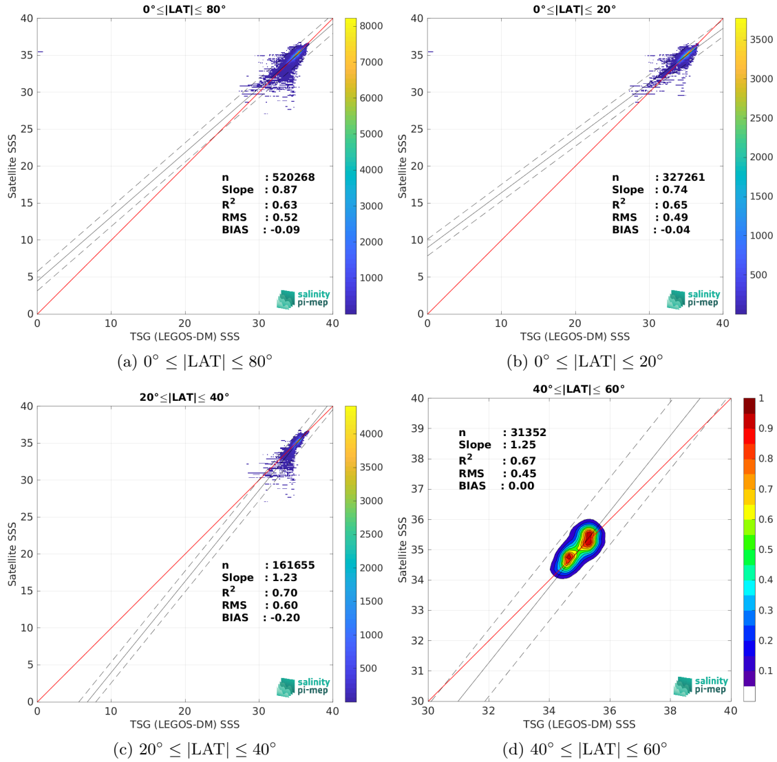
Figure 10: Contour maps of the concentration of Aquarius SSS L3 OR v5 - Monthly - Rain mask (NASA-GSFC) SSS (y-axis) versus TSG (LEGOS-DM) SSS (x-axis) at match-up pairs for different latitude bands. For each plot, the red line shows x=y . The black thin and dashed lines indicate a linear fit through the data cloud and the \pm 95\% confidence levels, respectively. The number match-up pairs n , the slope and R^2 coefficient of the linear fit, the root mean square (RMS) and the mean bias between satellite and in situ data are indicated for each latitude band in each plots.
