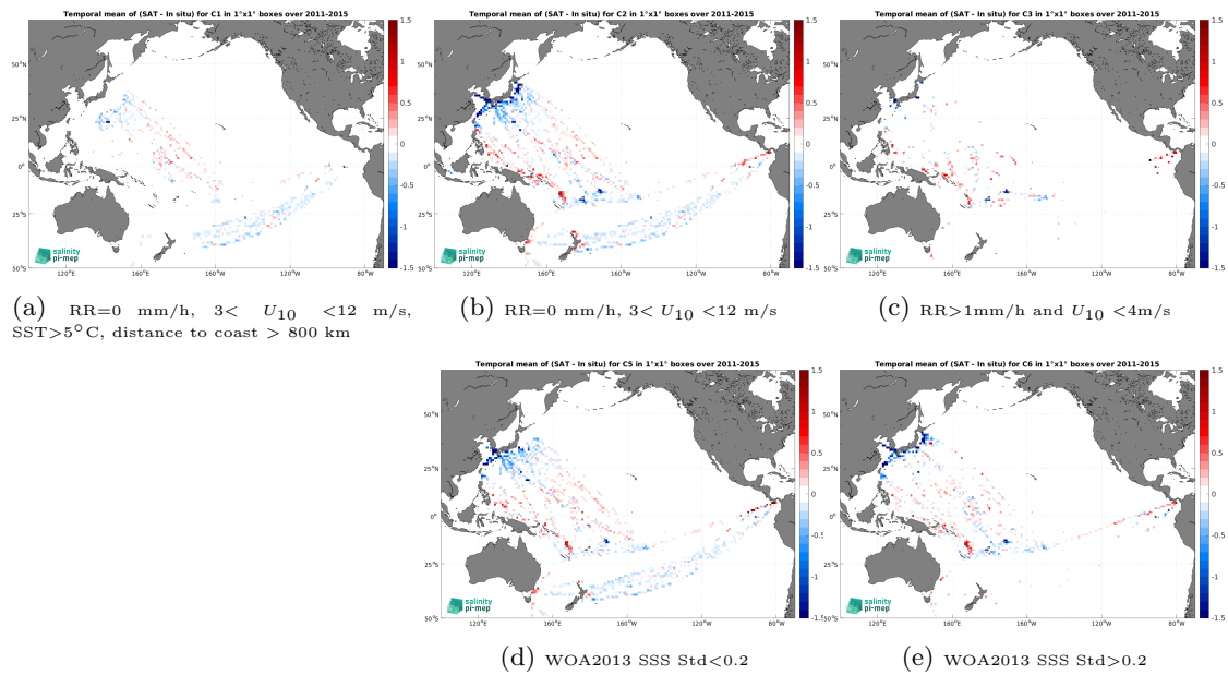
Figure 14: Temporal mean gridded over spatial boxes of size 1^\circ \times 1^\circ of \Delta\text{SSS} (Aquarius SSS L3 OR v5 - Monthly - Rain mask (NASA-GSFC) - TSG (LEGOS-DM)) for 5 different subdatasets corresponding to:RR=0 mm/h, 3 < U_{10} < 12 m/s, SST >5^\circ\text{C} , distance to coast > 800 km (a), RR=0 mm/h, 3 < U_{10} < 12 m/s (b), RR >1 mm/h and U_{10} < 4 m/s (c), WOA2013 SSS Std <0.2 (d), WOA2013 SSS Std >0.2 (e).
