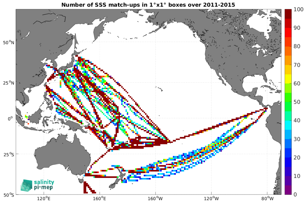
Figure 5: Number of SSS match-ups between TSG (LEGOS-DM) SSS and the Aquarius SSS L3 OR v5 - Monthly - Rain mask (NASA-GSFC) SSS product for the Pacific Ocean Pi-MEP region over 1^\circ \times 1^\circ boxes and for the full satellite product period.
