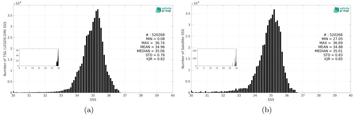
Figure 3: Histograms of SSS from TSG (LEGOS-DM) (a) and Aquarius SSS L3 OR v5 - Monthly - Rain mask (NASA-GSFC) (b) considering all match-up pairs per bins of 0.1 over the Pacific Ocean Pi-MEP region and for the full satellite product period.
