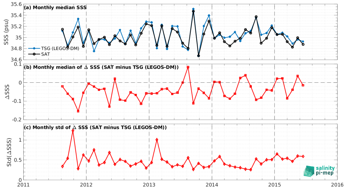
Figure 7: Time series of the monthly median SSS (top), median of \Delta\text{SSS} (Satellite - TSG (LEGOS-DM)) and \text{Std}(\Delta\text{SSS}) (Satellite - TSG (LEGOS-DM)) over the Pacific Ocean Pi-MEP region considering all match-ups collected by the Pi-MEP.
