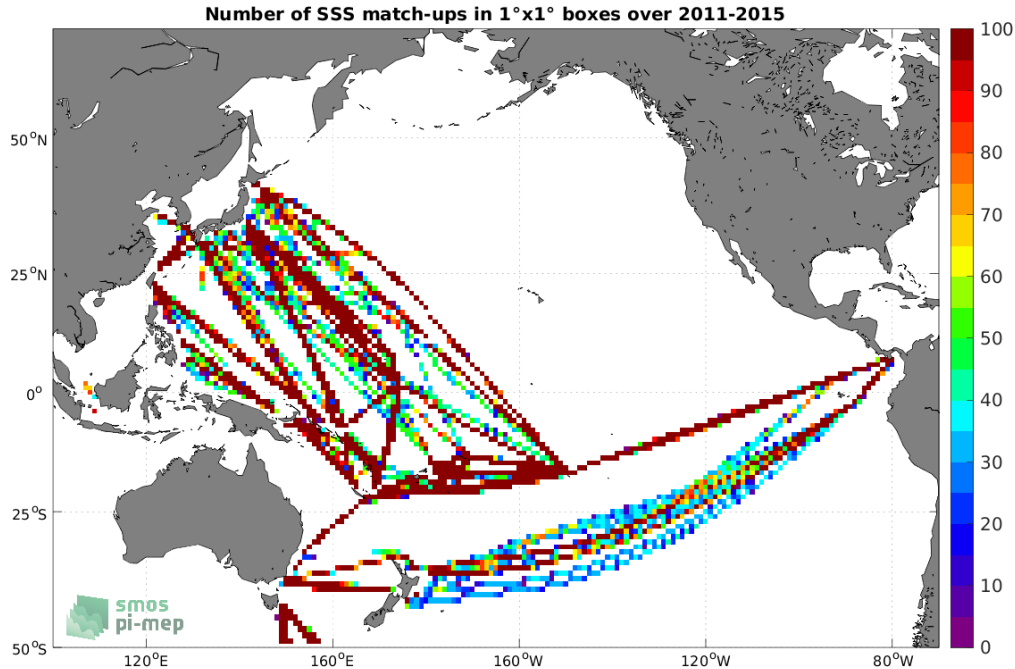
Figure 4: Number of SSS match-ups between TSG (LEGOS-DM) SSS and the Aquarius SSS L3 OR v5 - Monthly - Rain mask (NASA-GSFC) SSS product for the Pacific Ocean Pi-MEP region over 1^\circ \times 1^\circ boxes and for the full satellite product period.
