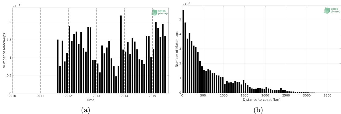
Figure 1: Number of match-ups between TSG (LEGOS-DM) and Aquarius SSS L3 OR v5 - Monthly - Rain mask (NASA-GSFC) SSS as a function of time (a) and as function of the distance to coast (b) over the Pacific Ocean Pi-MEP region and for the full satellite product period.
