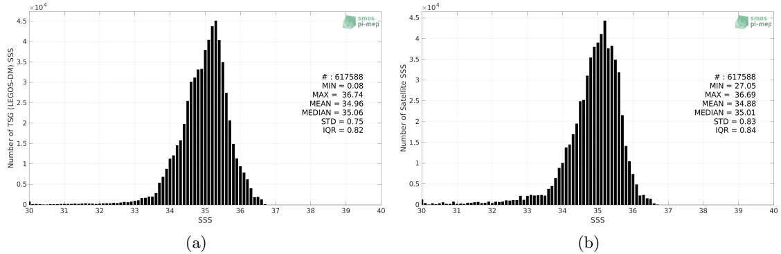
Figure 2: Histograms of SSS from TSG (LEGOS-DM) (a) and Aquarius SSS L3 OR v5 - Monthly - Rain mask (NASA-GSFC) (b) considering all match-up pairs per bins of 0.1 over the Pacific Ocean Pi-MEP region and for the full satellite product period.
