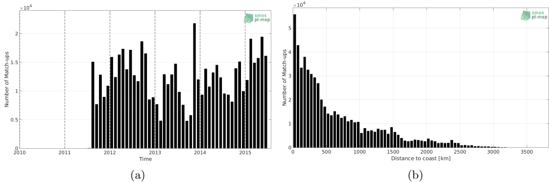
Figure 1: Number of match-ups between TSG-LEGOS-DM and Aquarius-L3-OR-V5-MONTHLY-RAIN-MASK-1DEG SSS as a function of time (a) and as function of the distance to coast (b) over the Pacific Ocean Pi-MEP region and for the full satellite product period.
