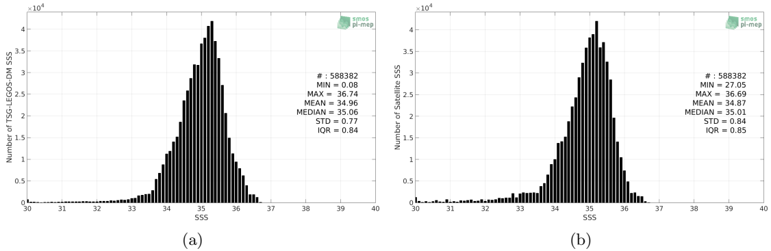
Figure 2: Histograms of SSS from TSG-LEGOS-DM (a) and Aquarius-L3-OR-V5-MONTHLY-RAIN-MASK-1DEG (b) considering all match-up pairs per bins of 0.1 over the Pacific Ocean Pi-MEP region and for the full satellite product period.
