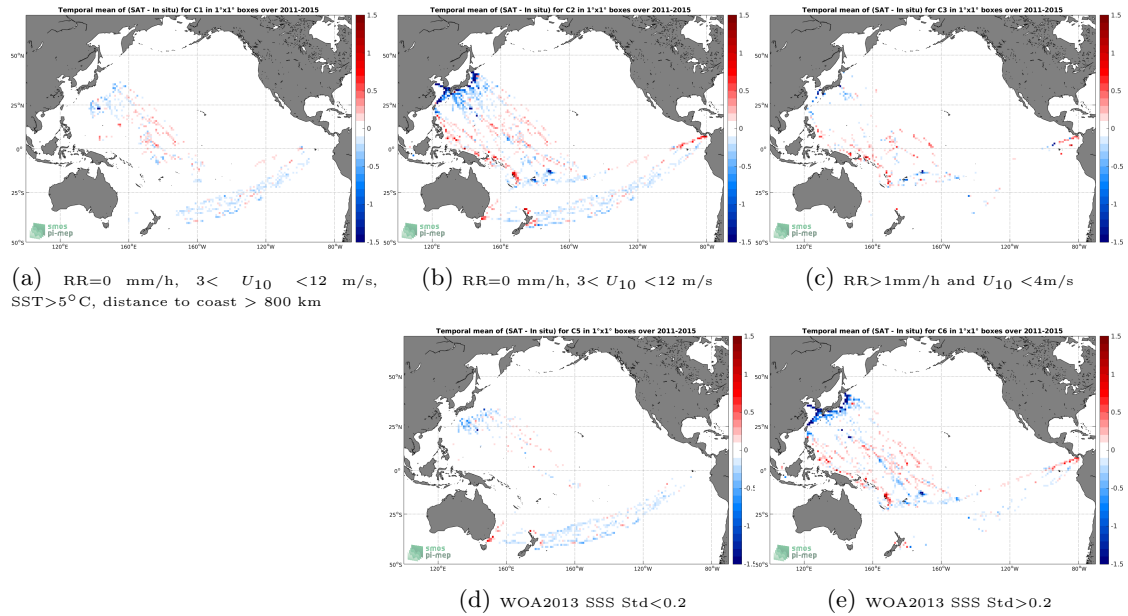
Figure 12: Temporal mean gridded over spatial boxes of size 1^\circ \times 1^\circ of \Delta SSS (Aquarius-L3-OR-V5-MONTHLY-RAIN-MASK-1DEG - TSG-LEGOS-DM) for 5 different subdatasets corresponding to:RR=0 mm/h, 3 < U_{10} < 12 m/s, SST >5^\circ C, distance to coast > 800 km (a), RR=0 mm/h, 3 < U_{10} < 12 m/s (b), RR >1 mm/h and U_{10} < 4 m/s (c), WOA2013 SSS Std <0.2 (d), WOA2013 SSS Std >0.2 (e).
