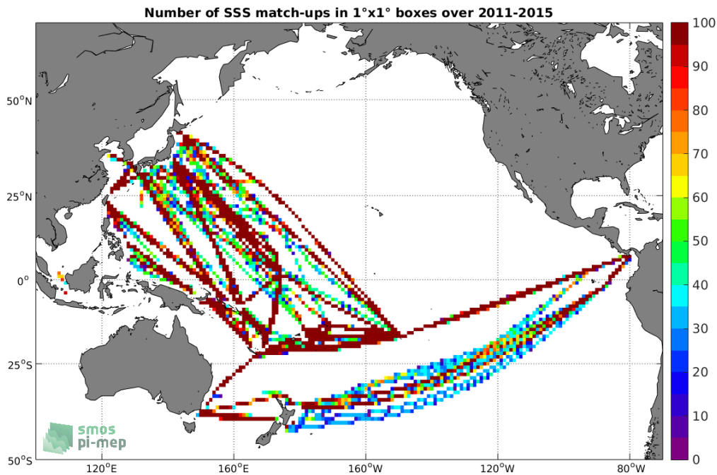
Figure 4: Number of SSS match-ups between TSG-LEGOS-DM SSS and the Aquarius-L3-OR-V5-MONTHLY-RAIN-MASK-1DEG SSS product for the Pacific Ocean Pi-MEP region over 1^\circ \times 1^\circ boxes and for the full satellite product period.
