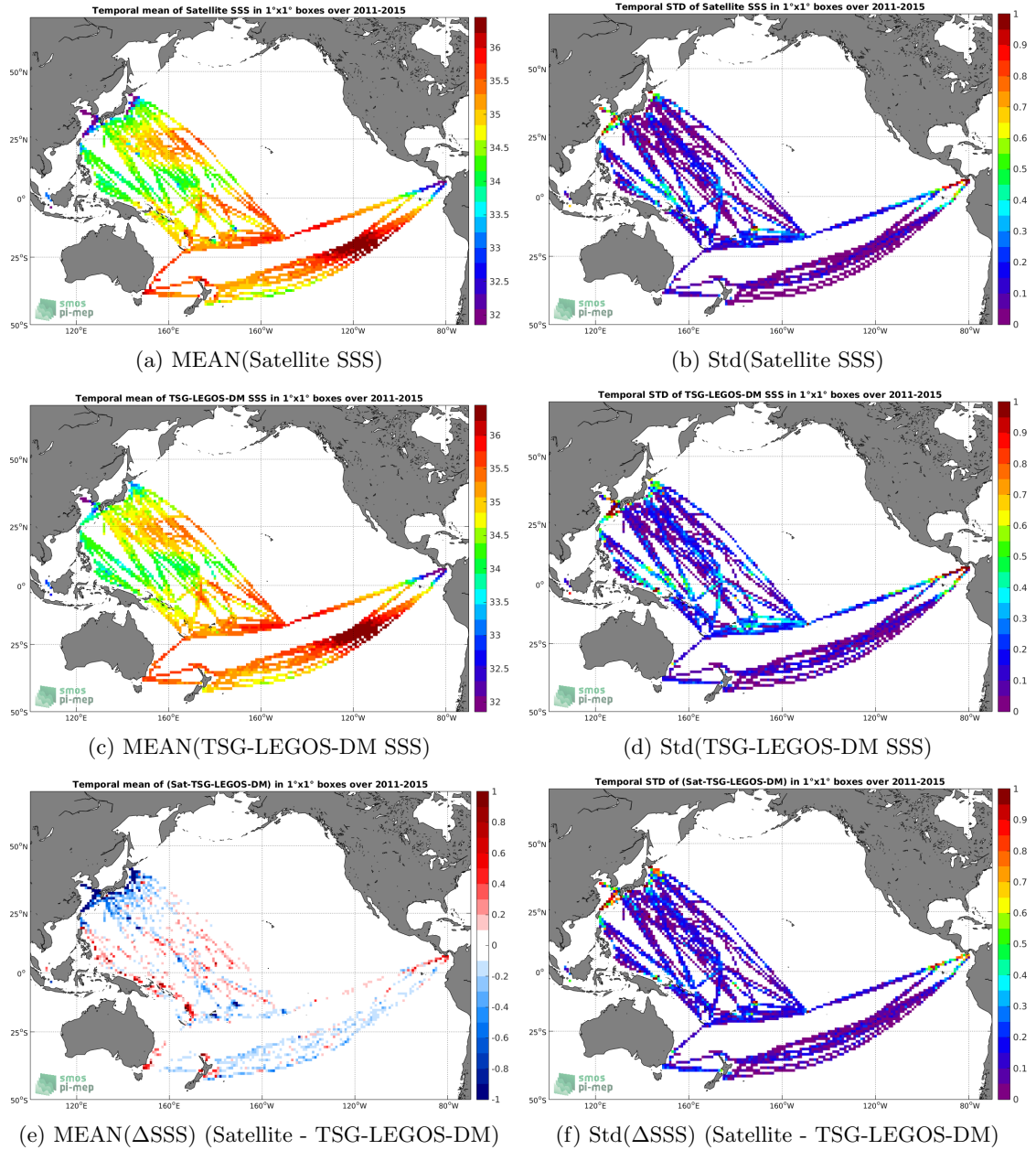
Figure 6: Temporal mean (left) and Std (right) of SSS from Aquarius-L3-OR-V5-MONTHLY-RAIN-MASK-1DEG (top), TSG-LEGOS-DM (middle), and of \Delta SSS (Satellite - TSG-LEGOS-DM). Only match-up pairs are used to generate these maps.
