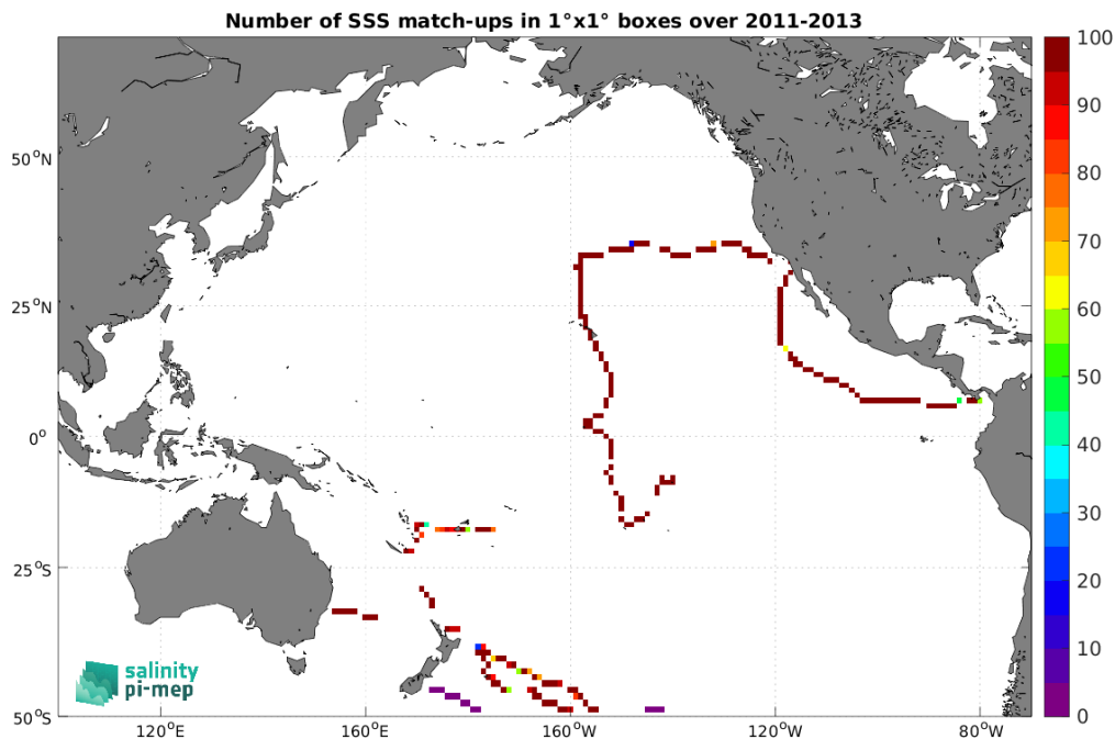
Figure 5: Number of SSS match-ups between TSG (GOSUD-Sailing-ship) SSS and the Aquarius SSS L3 OR v5 - Monthly - Rain mask (NASA-GSFC) SSS product for the Pacific Ocean Pi-MEP region over 1^\circ \times 1^\circ boxes and for the full satellite product period.
