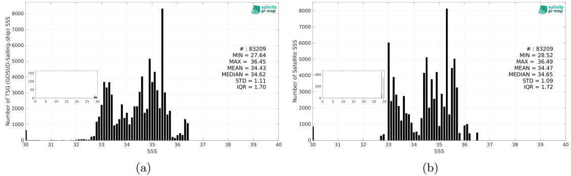
Figure 3: Histograms of SSS from TSG (GOSUD-Sailing-ship) (a) and Aquarius SSS L3 OR v5 - Monthly - Rain mask (NASA-GSFC) (b) considering all match-up pairs per bins of 0.1 over the Pacific Ocean Pi-MEP region and for the full satellite product period.
