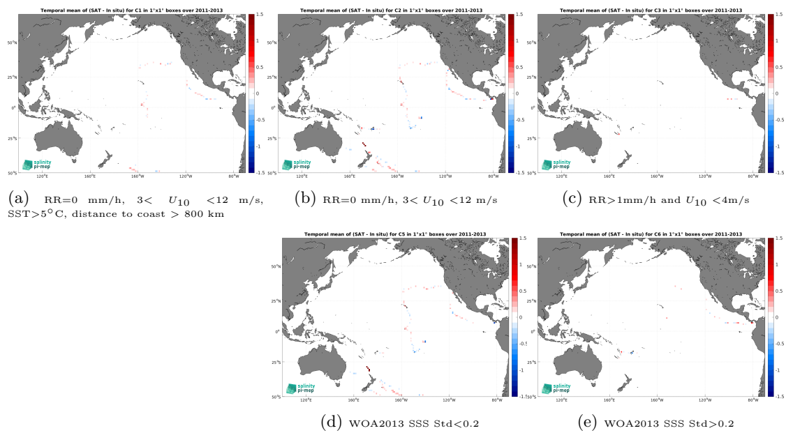
Figure 14: Temporal mean gridded over spatial boxes of size 1^\circ \times 1^\circ of \Delta SSS (Aquarius SSS L3 OR v5 - Monthly - Rain mask (NASA-GSFC) - TSG (GOSUD-Sailing-ship)) for 5 different subdatasets corresponding to:RR=0 mm/h, 3 < U_{10} < 12 m/s, SST >5^\circ\text{C} , distance to coast > 800 km (a), RR=0 mm/h, 3 < U_{10} < 12 m/s (b), RR >1 mm/h and U_{10} < 4 m/s (c), WOA2013 SSS Std <0.2 (d), WOA2013 SSS Std >0.2 (e).
