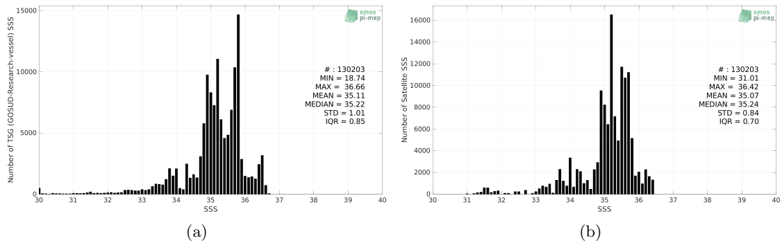
Figure 2: Histograms of SSS from TSG (GOSUD-Research-vessel) (a) and Aquarius SSS L3 OR v5 - Monthly - Rain mask (NASA-GSFC) (b) considering all match-up pairs per bins of 0.1 over the Pacific Ocean Pi-MEP region and for the full satellite product period.
