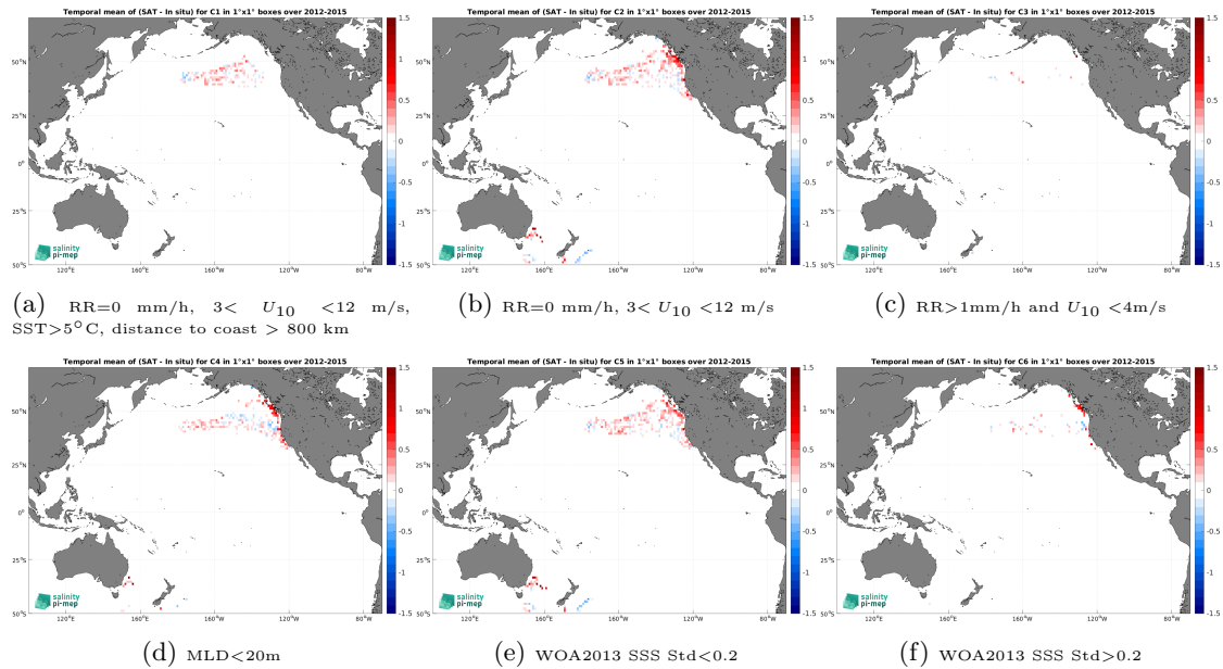
Figure 14: Temporal mean gridded over spatial boxes of size 1^\circ \times 1^\circ of \Delta SSS (Aquarius SSS L3 OR v5 - Monthly - Rain mask (NASA-GSFC) - Marine mammals) for 6 different subdatasets corresponding to: RR=0 mm/h, 3 < U_{10} < 12 m/s, SST > 5°C, distance to coast > 800 km (a), RR=0 mm/h, 3 < U_{10} < 12 m/s (b), RR > 1mm/h and U_{10} < 4 m/s (c), MLD < 20m (d), WOA2013 SSS Std < 0.2 (e), WOA2013 SSS Std > 0.2 (f).
