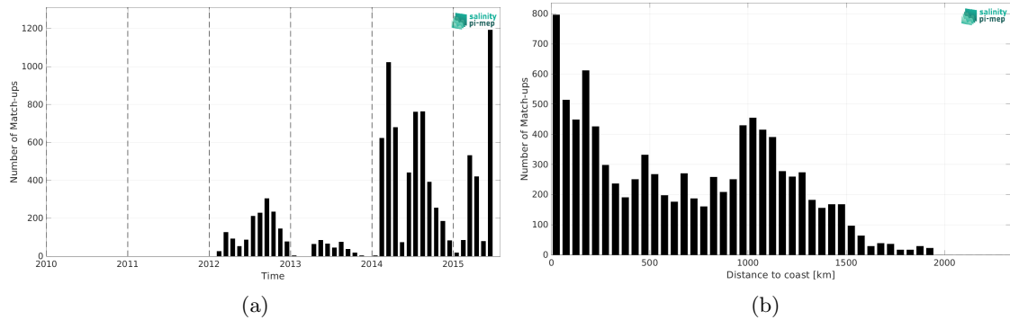
Figure 2: Number of match-ups between Marine mammals and Aquarius SSS L3 OR v5 - Monthly - Rain mask (NASA-GSFC) SSS as a function of time (a) and as function of the distance to coast (b) over the Pacific Ocean Pi-MEP region and for the full satellite product period.
