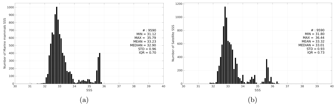
Figure 3: Histograms of SSS from Marine mammals (a) and Aquarius SSS L3 OR v5 - Monthly - Rain mask (NASA-GSFC) (b) considering all match-up pairs per bins of 0.1 over the Pacific Ocean Pi-MEP region and for the full satellite product period.
