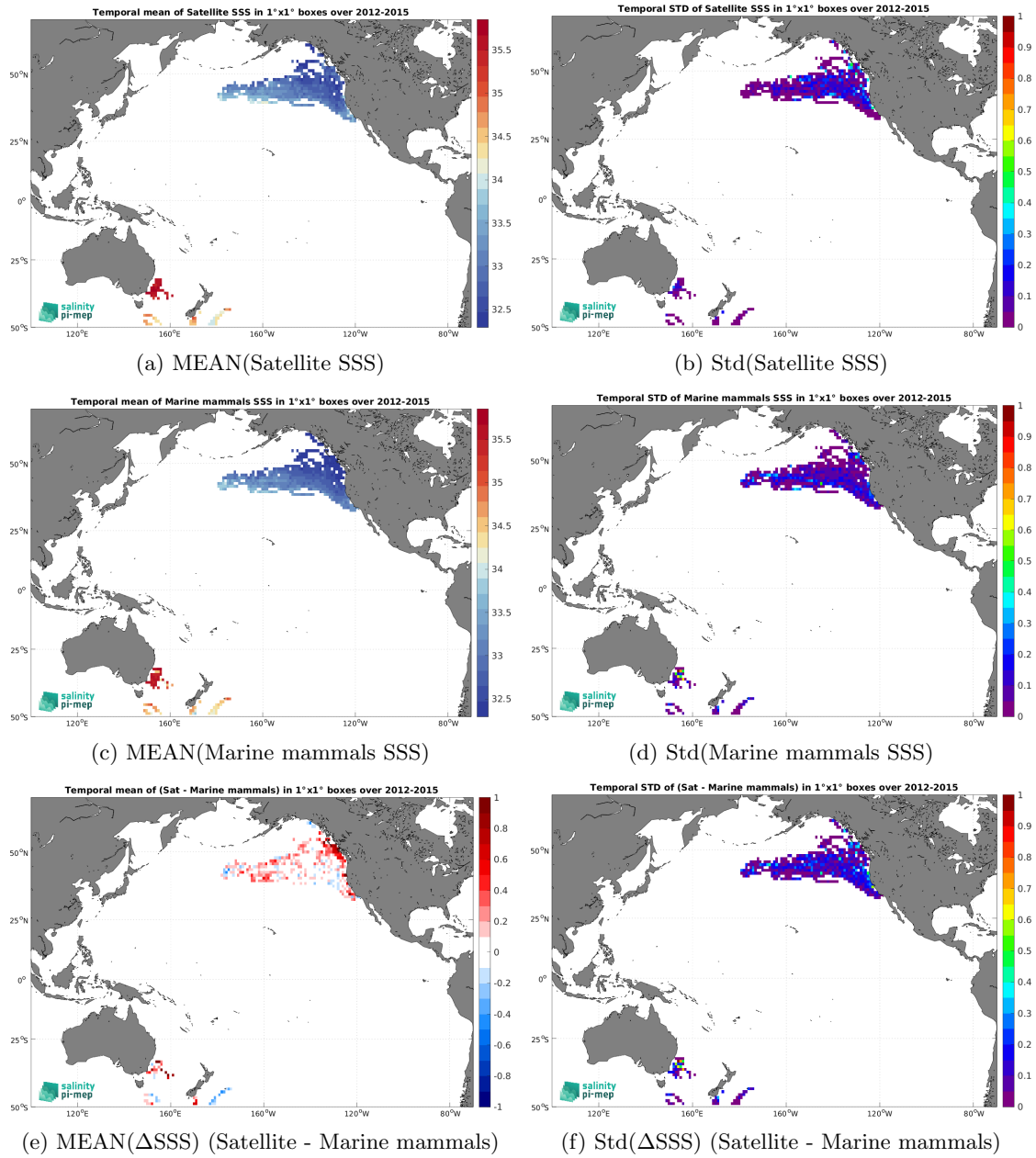
Figure 7: Temporal mean (left) and Std (right) of SSS from Aquarius SSS L3 OR v5 - Monthly - Rain mask (NASA-GSFC) (top), Marine mammals (middle), and of \Delta SSS (Satellite - Marine mammals). Only match-up pairs are used to generate these maps.
