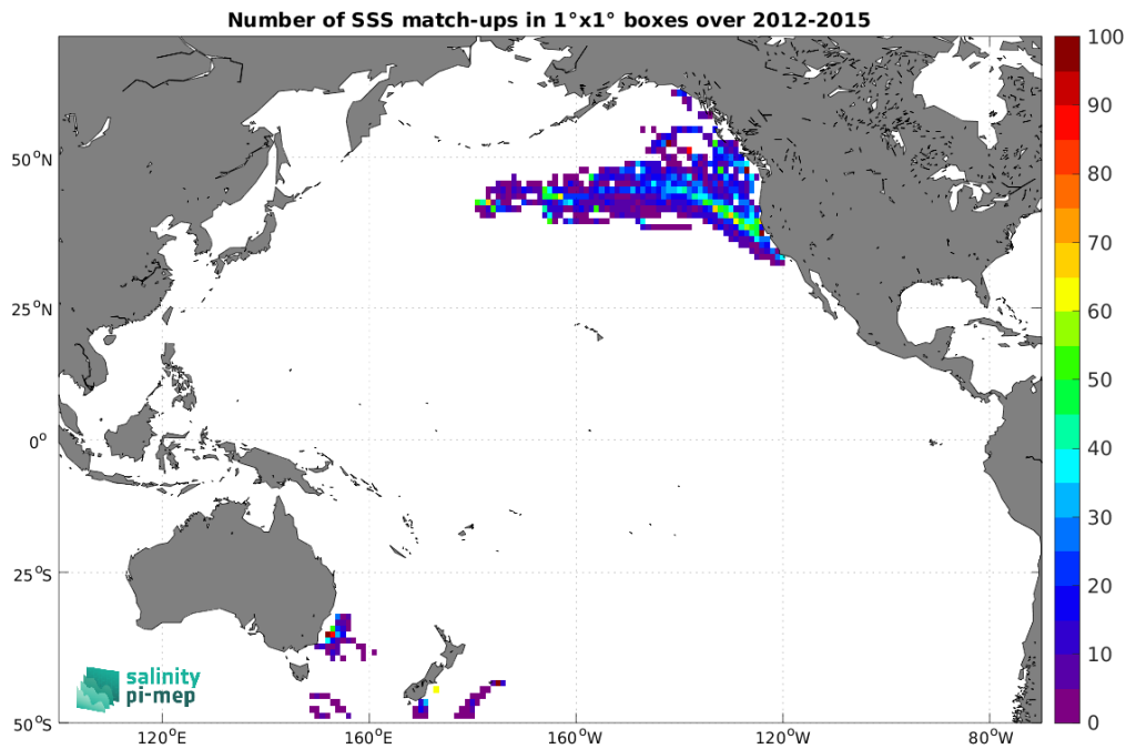
Figure 5: Number of SSS match-ups between Marine mammals SSS and the Aquarius SSS L3 OR v5 - Monthly - Rain mask (NASA-GSFC) SSS product for the Pacific Ocean Pi-MEP region over 1^\circ \times 1^\circ boxes and for the full satellite product period.
