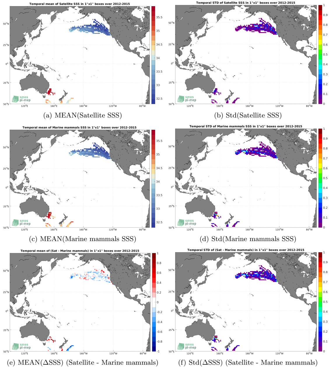
Figure 6: Temporal mean (left) and Std (right) of SSS from Aquarius SSS L3 OR v5 - Monthly - Rain mask (NASA-GSFC) (top), Marine mammals (middle), and of \Delta SSS (Satellite - Marine mammals). Only match-up pairs are used to generate these maps.
