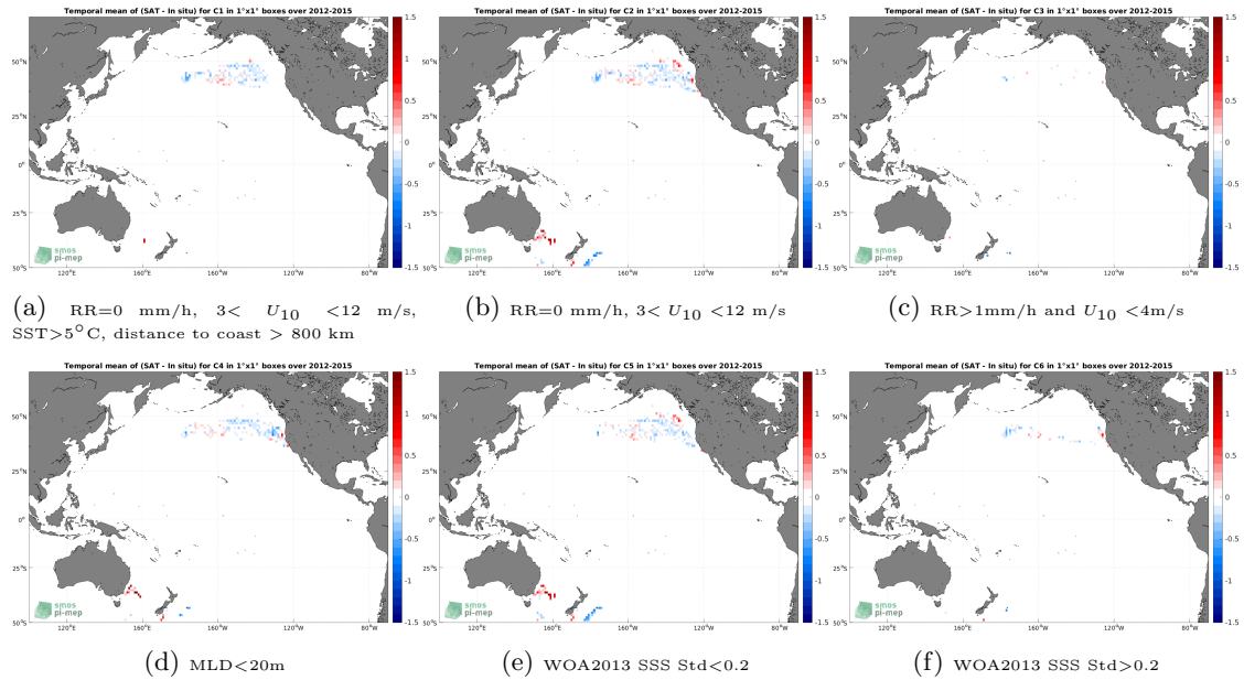
Figure 12: Temporal mean gridded over spatial boxes of size 1^{\circ}\times 1^{\circ} of \Delta\text{SSS} (Aquarius SSS L3 OR v5 - Monthly - Rain mask (NASA-GSFC) - Marine mammals) for 6 different subdatasets corresponding to: \text{RR}=0 mm/h, 3 < U_{10} < 12 m/s, \text{SST} > 5^{\circ}\text{C} , distance to coast > 800 km (a), \text{RR}=0 mm/h, 3 < U_{10} < 12 m/s (b), \text{RR} > 1\text{mm/h} and U_{10} < 4\text{m/s} (c), \text{MLD} < 20\text{m} (d), WOA2013 SSS Std < 0.2 (e), WOA2013 SSS Std > 0.2 (f).
