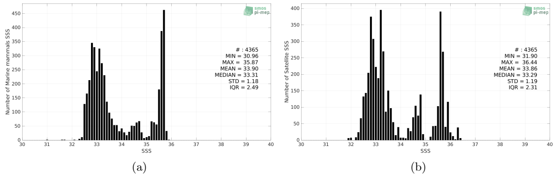
Figure 2: Histograms of SSS from Marine mammals (a) and Aquarius SSS L3 OR v5 - Monthly - Rain mask (NASA-GSFC) (b) considering all match-up pairs per bins of 0.1 over the Pacific Ocean Pi-MEP region and for the full satellite product period.
