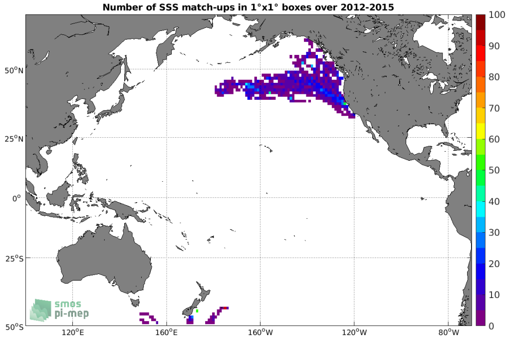
Figure 4: Number of SSS match-ups between Marine mammals SSS and the Aquarius SSS L3 OR v5 - Monthly - Rain mask (NASA-GSFC) SSS product for the Pacific Ocean Pi-MEP region over 1^{\circ} \times 1^{\circ} boxes and for the full satellite product period.
