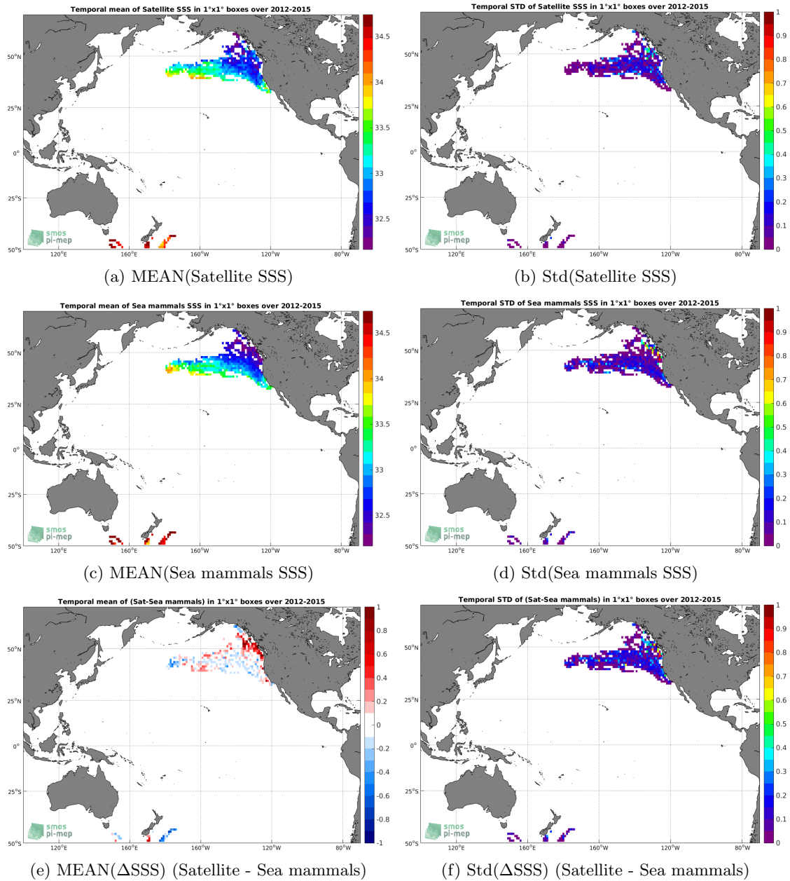
Figure 6: Temporal mean (left) and Std (right) of SSS from Aquarius-L3-OR-V5-MONTHLY-RAIN-MASK-1DEG (top), Sea mammals (middle), and of \Delta SSS (Satellite - Sea mammals). Only match-up pairs are used to generate these maps.
