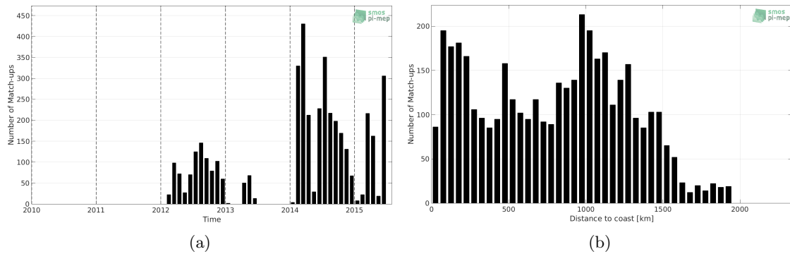
Figure 1: Number of match-ups between Sea mammals and Aquarius-L3-OR-V5-MONTHLY-RAIN-MASK-1DEG SSS as a function of time (a) and as function of the distance to coast (b) over the Pacific Ocean Pi-MEP region and for the full satellite product period.
