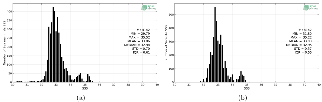
Figure 2: Histograms of SSS from Sea mammals (a) and Aquarius-L3-OR-V5-MONTHLY-RAIN-MASK-1DEG (b) considering all match-up pairs per bins of 0.1 over the Pacific Ocean Pi-MEP region and for the full satellite product period.
