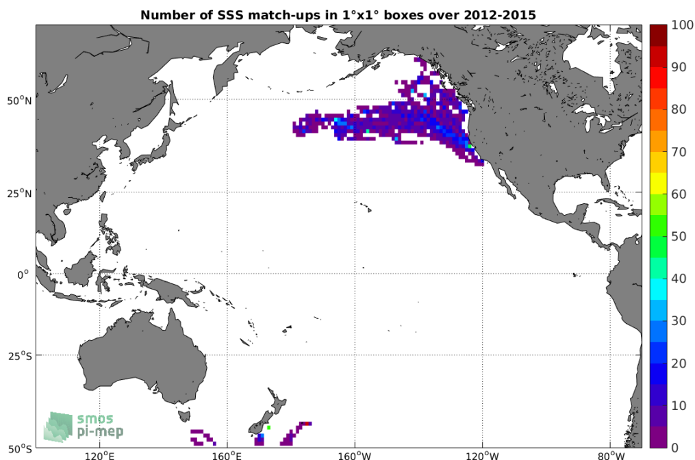
Figure 4: Number of SSS match-ups between Sea mammals SSS and the Aquarius-L3-OR-V5-MONTHLY-RAIN-MASK-1DEG SSS product for the Pacific Ocean Pi-MEP region over 1°x1° boxes and for the full satellite product period.
