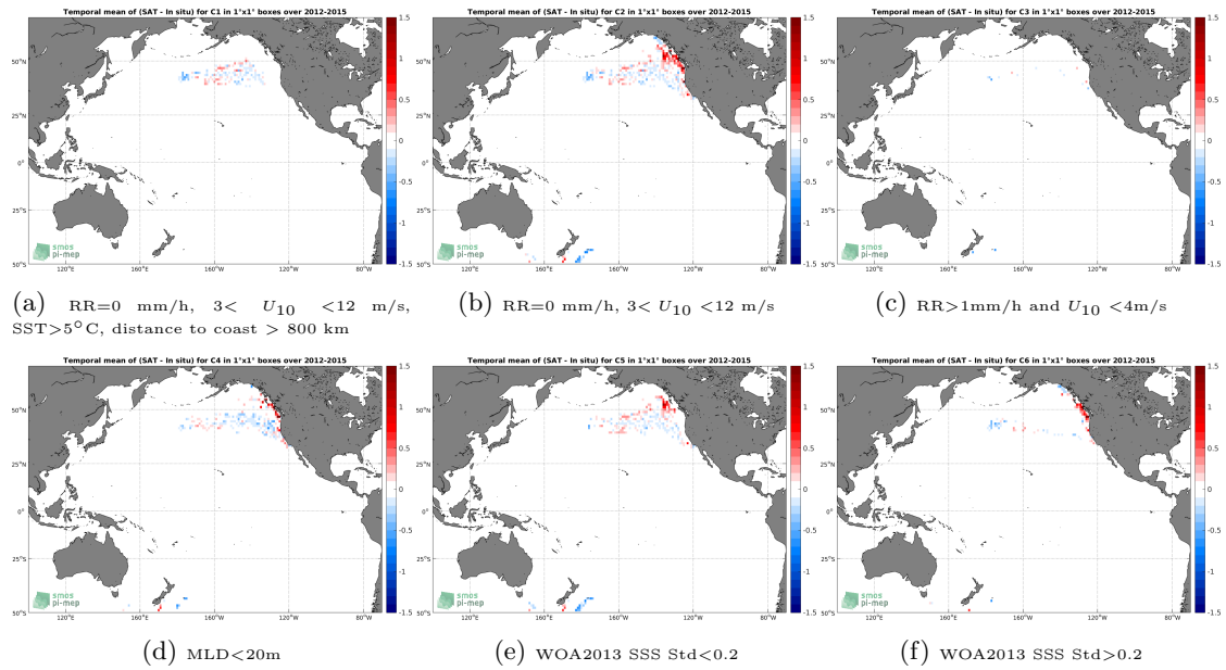
Figure 12: Temporal mean gridded over spatial boxes of size 1^\circ \times 1^\circ of \Delta SSS (Aquarius-L3-OR-V5-MONTHLY-RAIN-MASK-1DEG - Sea mammals) for 6 different subdatasets corresponding to:RR=0 mm/h, 3 < U_{10} < 12 m/s, SST >5^\circ C, distance to coast > 800 km (a), RR=0 mm/h, 3 < U_{10} < 12 m/s (b), RR >1 mm/h and U_{10} < 4 m/s (c),MLD <20 m (d),WOA2013 SSS Std <0.2 (e),WOA2013 SSS Std >0.2 (f).
