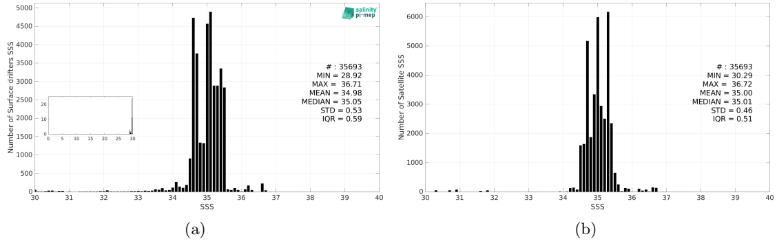
Figure 3: Histograms of SSS from Surface drifters (a) and Aquarius SSS L3 OR v5 - Monthly - Rain mask (NASA-GSFC) (b) considering all match-up pairs per bins of 0.1 over the Pacific Ocean Pi-MEP region and for the full satellite product period.
