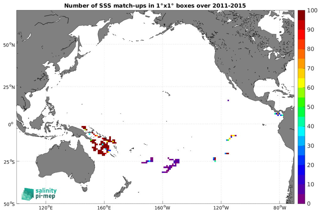
Figure 4: Number of SSS match-ups between Surface drifters SSS and the Aquarius SSS L3 OR v5 - Monthly - Rain mask (NASA-GSFC) SSS product for the Pacific Ocean Pi-MEP region over 1^\circ \times 1^\circ boxes and for the full satellite product period.
