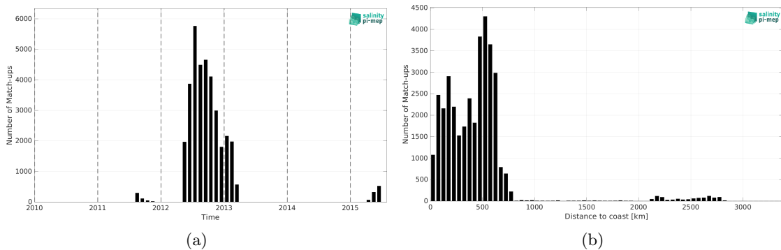
Figure 2: Number of match-ups between Surface drifters and Aquarius SSS L3 OR v5 - Monthly - Rain mask (NASA-GSFC) SSS as a function of time (a) and as function of the distance to coast (b) over the Pacific Ocean Pi-MEP region and for the full satellite product period.
