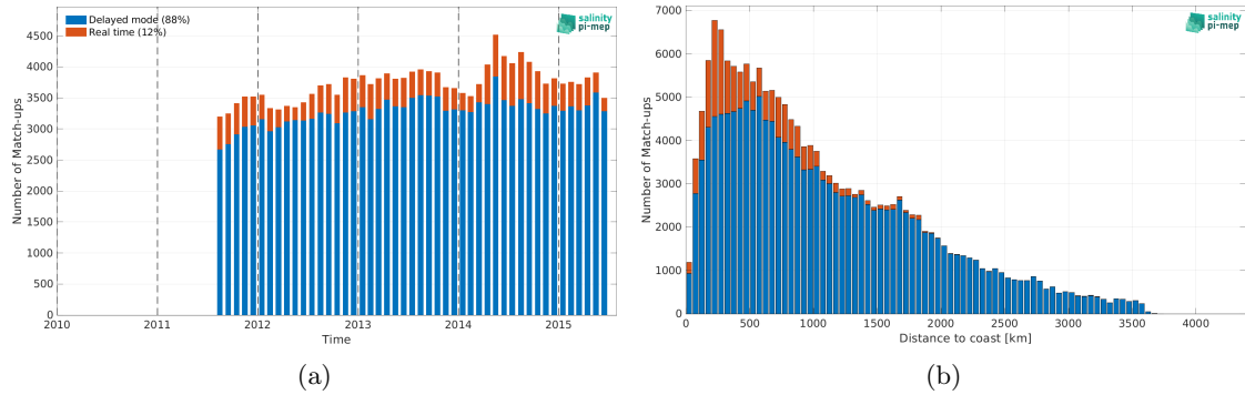
Figure 2: Number of match-ups between Argo and Aquarius SSS L3 OR v5 - Monthly - Rain mask (NASA-GSFC) SSS as a function of time (a) and as function of the distance to coast (b) over the Pacific Ocean Pi-MEP region and for the full satellite product period.
