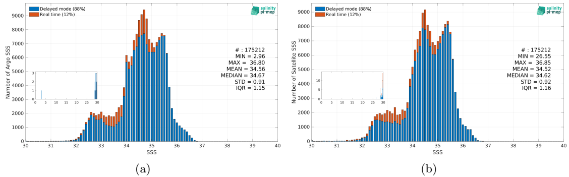
Figure 3: Histograms of SSS from Argo (a) and Aquarius SSS L3 OR v5 - Monthly - Rain mask (NASA-GSFC) (b) considering all match-up pairs per bins of 0.1 over the Pacific Ocean Pi-MEP region and for the full satellite product period.
