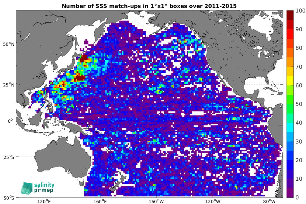
Figure 5: Number of SSS match-ups between Argo SSS and the Aquarius SSS L3 OR v5 - Monthly - Rain mask (NASA-GSFC) SSS product for the Pacific Ocean Pi-MEP region over 1^\circ \times 1^\circ boxes and for the full satellite product period.
