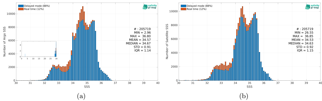
Figure 2: Histograms of SSS from Argo (a) and Aquarius SSS L3 OR v5 - Monthly - Rain mask (NASA-GSFC) (b) considering all match-up pairs per bins of 0.1 over the Pacific Ocean Pi-MEP region and for the full satellite product period.
