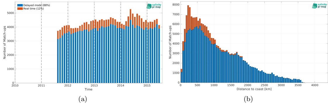
Figure 1: Number of match-ups between Argo and Aquarius SSS L3 OR v5 - Monthly - Rain mask (NASA-GSFC) SSS as a function of time (a) and as function of the distance to coast (b) over the Pacific Ocean Pi-MEP region and for the full satellite product period.
