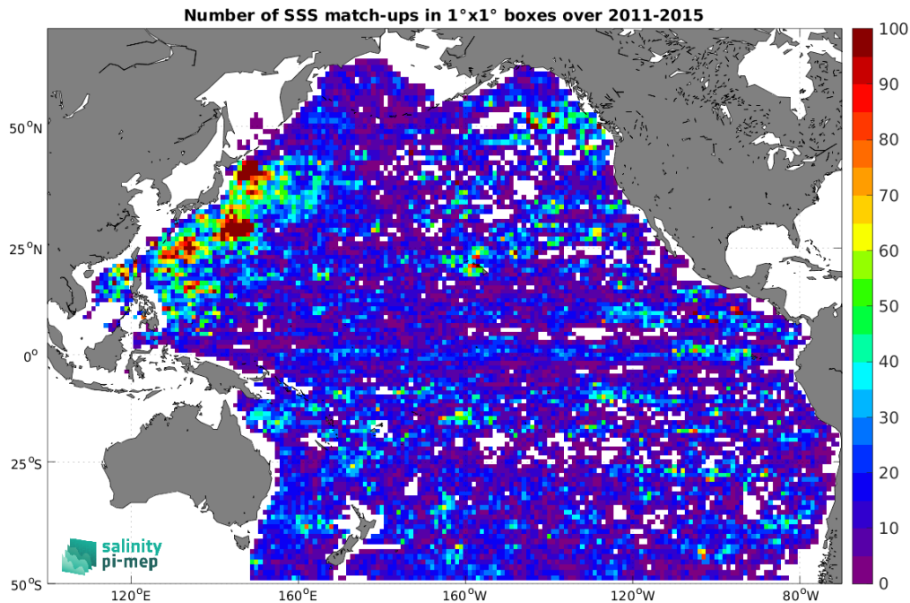
Figure 4: Number of SSS match-ups between Argo SSS and the Aquarius SSS L3 OR v5 - Monthly - Rain mask (NASA-GSFC) SSS product for the Pacific Ocean Pi-MEP region over 1^\circ \times 1^\circ boxes and for the full satellite product period.
