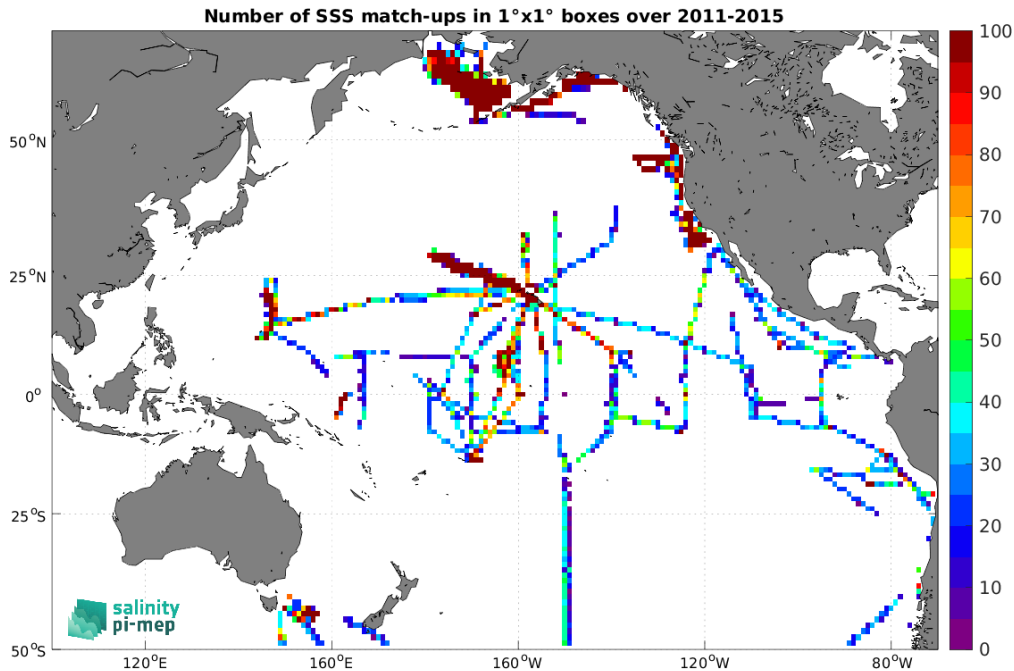
Figure 4: Number of SSS match-ups between TSG (SAMOS) SSS and the Aquarius SSS L3 CAP v5 - 7-Day running (JPL) SSS product for the Pacific Ocean Pi-MEP region over 1^\circ \times 1^\circ boxes and for the full satellite product period.
